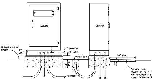
BASE MOUNTED CABINET
