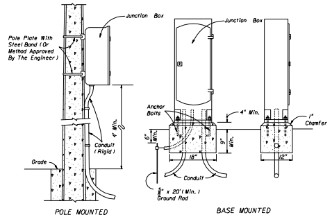
POLE MOUNTED
