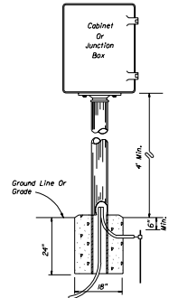
PEDESTAL MOUNTED
