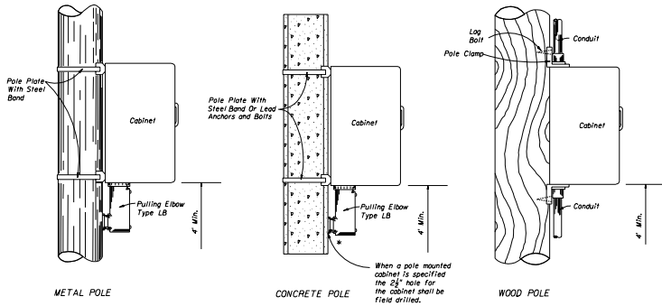
METAL POLE
