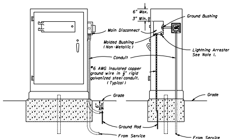
FIGURE E UNDERGROUND CABINET MOUNTED (METER USED)
