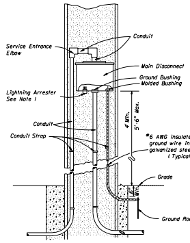
FIGURE C UNDERGROUND FEED (NO METER USED)
