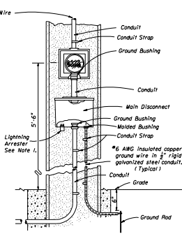
FIGURE B AERIAL FEED (METER USED)
