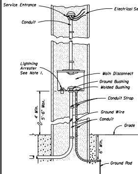
FIGURE A AERIAL FEED (NO METER USED)
