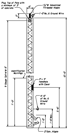
TYPE N-II POLE ON CONCRETE PEDESTAL
