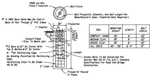
METAL POLE CONCRETE FOUNDATION DETAIL
