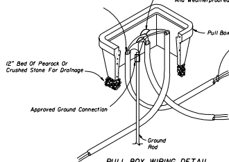
PULL BOX WIRING DETAIL
