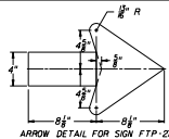
ARROW DETAIL FOR SIGN FTP-27
