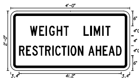
FTP - 50 5' x 2' 1\frac{1}{2} " Radii \frac{3}{4} " Border 4" Series C Yellow Background Black Legend & Border
