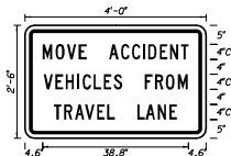
FTP - 46 4' X 2'-6" 2" Radii ¾" Border 4" Series C Legend White Background Black Legend & Border
