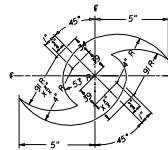
DETAIL 'A' for FTP - 53
