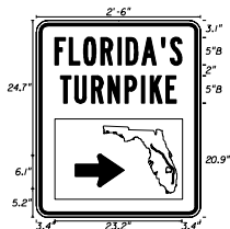
FTP - 27 1'-6" X 3" 1 1/2" Radii 3/4" Border Green Background White Legend & Border
