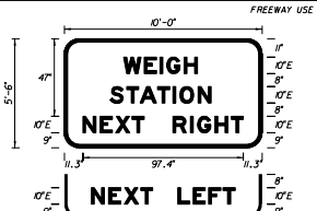
FTP - 5 10' X 5'-6" 3" Radii 2" Border 10" Series E Legend Green Background White Legend & Border
