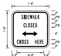
MOT - 8 1'-6" X 1'-6" 2 1/2" Radii 3/4" Border 2" Series B Legend White Background Black Legend & Border
