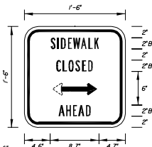
MOT - 5 1'-6" X 1'-6" 2" Radii 3/4" Border 2" Series B Legend White Background Black Legend & Border
