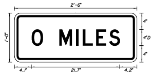
FTP - 51 3' x 1' 1\frac{1}{2} " Radii \frac{3}{4} " Border 4" Series D White Background Black Legend & Border
