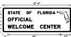
FTP - 15B 12'-6" X 7' 3" Radii 2" Border Series E Legend Green Background White Legend & Border
