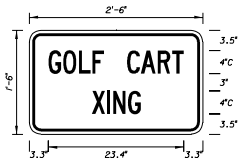
FTP - 39A 2'-6" X 1'-6" 1½" Radii ¾" Border 4" Series C Legend Yellow Background Black Legend & Border
