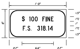
FTP - 55 1' x 6" 1\frac{1}{2} " Radii \frac{3}{4} " Border 1" Series C White Background Black Legend & Border Supplemental panel for the FTP-25 and FTP-26 signs
