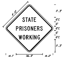
MOT - 11 4' x 4' 3" Radii 3/4" Border 6" Series C Legend Orange Background Black Legend & Border
