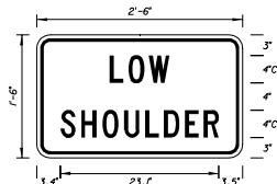
FTP - 42 2'-6" X 1'-6" 1½" Radii ¾" Border 4" Series C Legend Yellow Background Black Legend & Border
