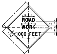
W20-1B LEGEND AND BORDER: BLACK BACKGROUND: ORANGE
