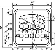
FTP - 61 24" x 24" 1 1/2" Radii 3/4" Border Blue Background White Legend & Border
