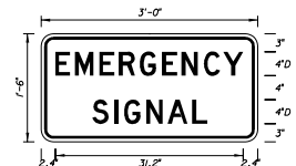
FTP - 45 3' X 1'-6" 1½" Radii ¾" Border 4" Series D Legend Yellow Background Black Legend & Border
