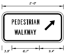
MOT - 6 2' x 1' 1 1/2" Radii 3/4" Border 2" Series B Legend White Background Black Legend & Border
