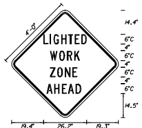
MOT - 10 4' x 4' 3" Radii 3/4" Border 6" Series C Legend Orange Background Black Legend & Border
