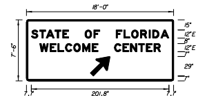
FTP - 18 18' X 7'-6" 3" Radii 2" Border Series E Legend Blue Background White Legend & Border
