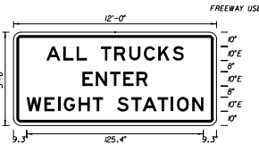
FTP - 4 12' X 5'-6" 3" Radii 2" Border 10" Series E Legend White Background Black Legend & Border
