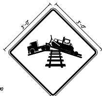
FTP - 40 3' X 3' 2" Radii ¾" Border Yellow Background Black Legend & Border
