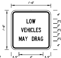
FTP - 40A 1'-6" X 1'-6" 1½" Radii ¾" Border 2" Series C Legend Yellow Background Black Legend & Border
