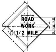
W20-1D LEGEND AND BORDER: BLACK BACKGROUND: ORANGE
