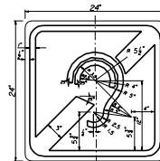
FTP - 60 24" x 24" 1 1/2" Radii 3/4" Border Blue Background White Legend & Border
