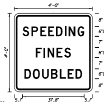
FTP - 56 Freeway Sign 4' x 4' 3" Radii \frac{3}{4} " Border 6" Series D White Background Black Legend & Border
