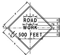
W20-1A LEGEND AND BORDER: BLACK BACKGROUND: ORANGE
