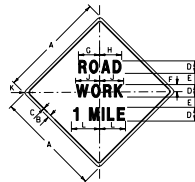
W20-1E LEGEND AND BORDER: BLACK BACKGROUND: ORANGE
