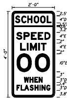
FTP - 37 2' X 4' 1 1/2" Radii 3/4" Border Top Background Yellow Bottom Background White Black Legend & Border Top and Bottom
