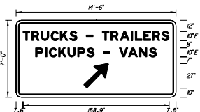
FTP - 16 14'-6" X 7' 3" Radii 2" Border Series E Legend Green Background White Legend & Border
