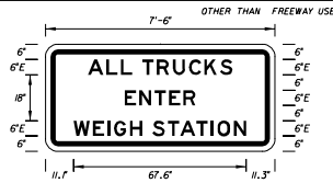
FTP - 8 7'-6" X 3'-6" 3" Radii 2" Border 6" Series E Legend White Background Black Legend & Border
