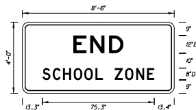
FTP - 34 8'-6" X 4' 3" Radii 3/4" Border White Background Black Legend & Border
