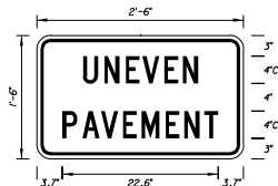
FTP - 43 2'-6" X 1'-6" 1½" Radii ¾" Border 4" Series C Legend Yellow Background Black Legend & Border
