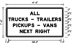
FTP - 14A 14'-6" X 7'-6" 3" Radii 2" Border 10" Series E Legend White Background Black Legend & Border
