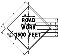
W20-1C LEGEND AND BORDER: BLACK BACKGROUND: ORANGE
