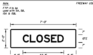
FTP - 11 7' X 2' 1/4" Radii 2" Border 10" Series E Legend Green Background White Legend & Border
