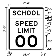
FTP - 44 2'-6" X 3' 1½" Radii ¾" Border Series E Legend Yellow Background Top White Background Bottom Black Legend & Border
