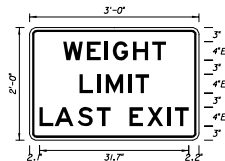
FTP - 52 3' x 2' 1\frac{1}{2} " Radii \frac{3}{4} " Border 4" Series C White Background Black Legend & Border
