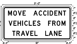
FTP - 46A 9' X 4'-6" 3" Radii ¾" Border 8" Series D Legend White Background Black Legend & Border
