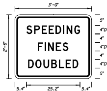
FTP - 57 Arterial Sign 3' x 2'-6" 2" Radii 3/4" Border 4" Series D White Background Black Legend & Border
