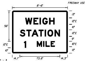
FTP - 3 8'-6" X 5'-6" 3" Radii 2" Border Series E Legend Green Background White Legend & Border
