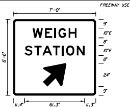
FTP - 6 7' X 6'-6" 3" Radii 2" Border 10" Series E Legend Green Background White Legend & Border
