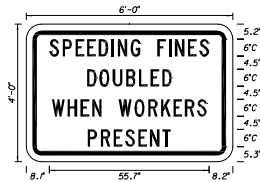
MOT - 14 6' X 4' 3" Radii \frac{3}{4} " Border 6" Series C Legend White Background Black Legend & Border
