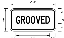
FTP - 41 2' X 1' 1½" Radii ¾" Border 4" Series C Legend Yellow Background Black Legend & Border
