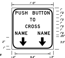
FTP - 48 1' x 1' 1\frac{1}{2} " Radii \frac{3}{4} " Border 1" Series D Legend White Background Black Legend & Border
