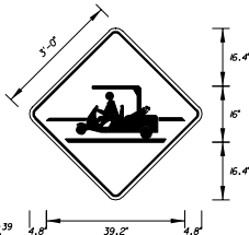
FTP - 39 3' X 3' 2" Radii 3/4" Border Yellow Background Black Legend & Border
