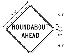
FTP - 54 3' x 3' 2" Radii \frac{3}{4} " Border 5" Series D Yellow Background Black Legend & Border
