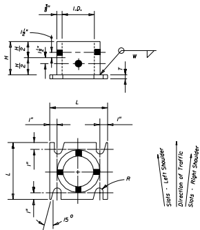
SLEEVE & BASE PLATE DETAILS
