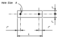
0.04" Thick Alum. Slip-2 Req'd Per Base BOLT KEEPER DETAIL
