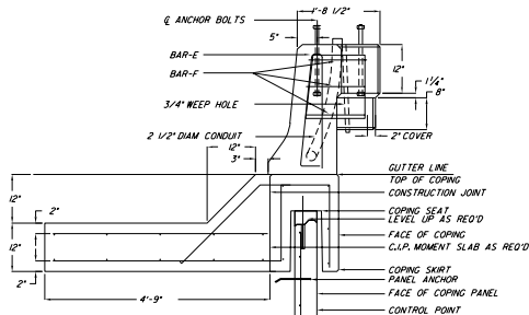
A B PRECAST COPING WITH PILASTER SECTION
