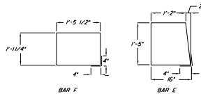
REBAR SCHEDULE
