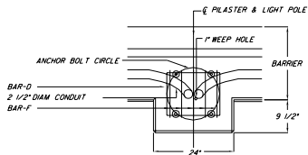
B 8 PILASTER PLAN VIEW
