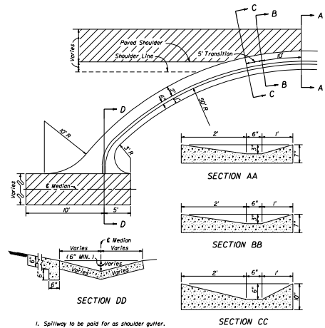
DETAIL OF CONC. SPILLWAY AT END OF SHOULDER GUTTER (TO BE USED WHERE INLETS, PIPES & ENDWALLS ARE IMPRACTICAL)
