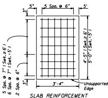
SLAB REINFORCEMENT
