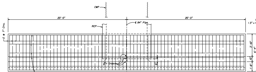
PLAN (Showing Bars in Footing)
