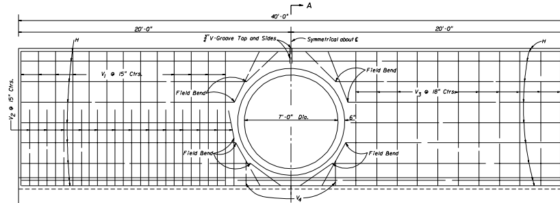
HALF ELEVATION
