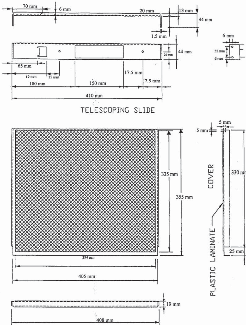
FIGURE 676-26 STORAGE COMPARTMENT TELESOPING SLIDE AND COVER DETAIL
