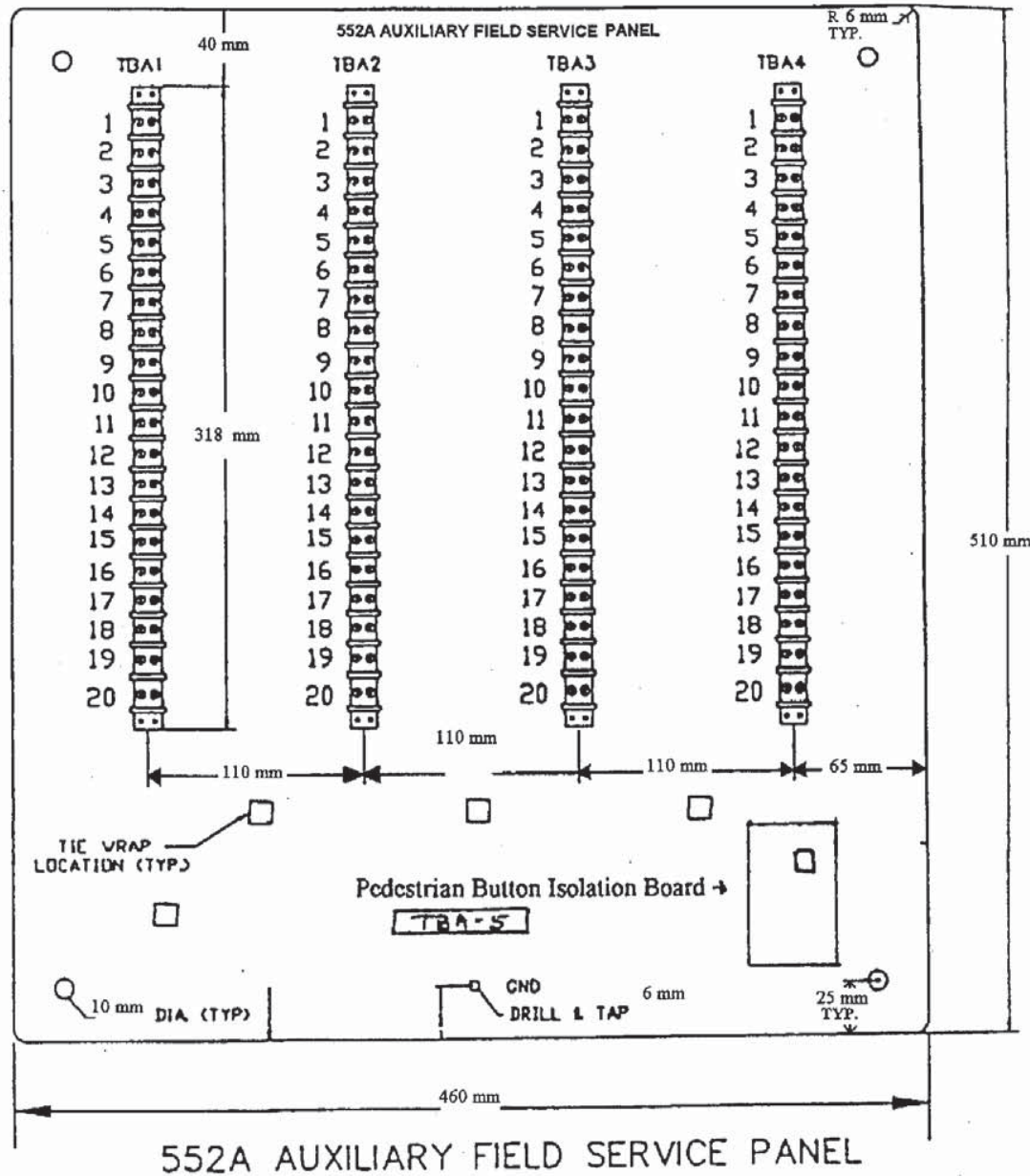
FIGURE 676-38 AUXILIARY FIELD SERVICE PANEL LAYOUT
