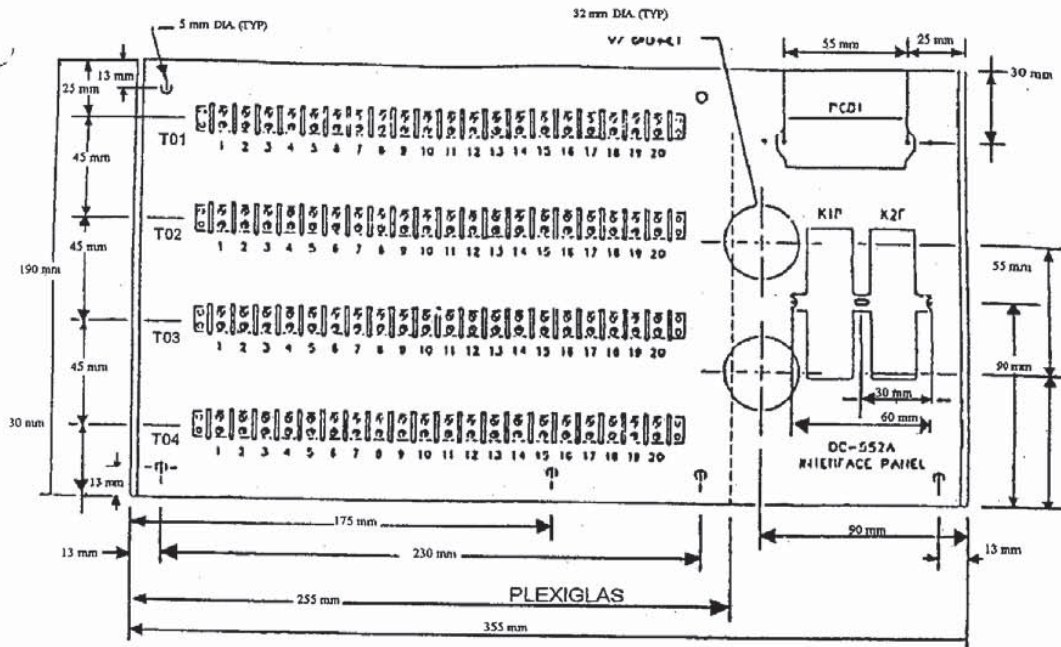
FIGURE 676-41 INTERFACE PANEL LAYOUT
