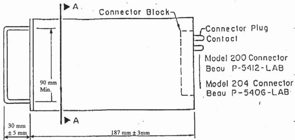
FIGURE 678-7 MODEL 200 SWITCH PACK & MODEL 204 FLASHER DETAILS
