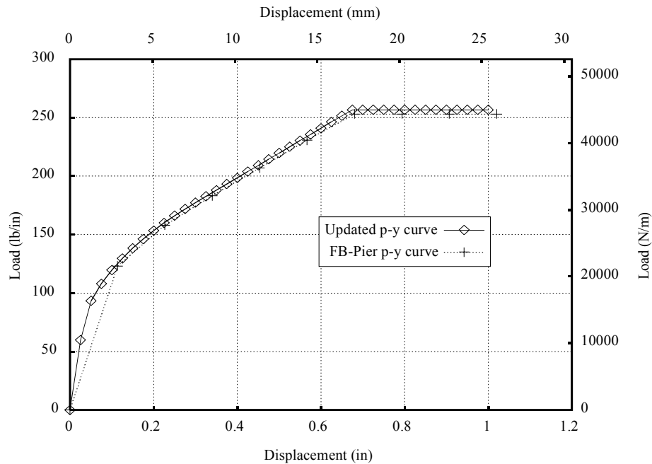
Figure 5.1. PY-Curve Comparison
