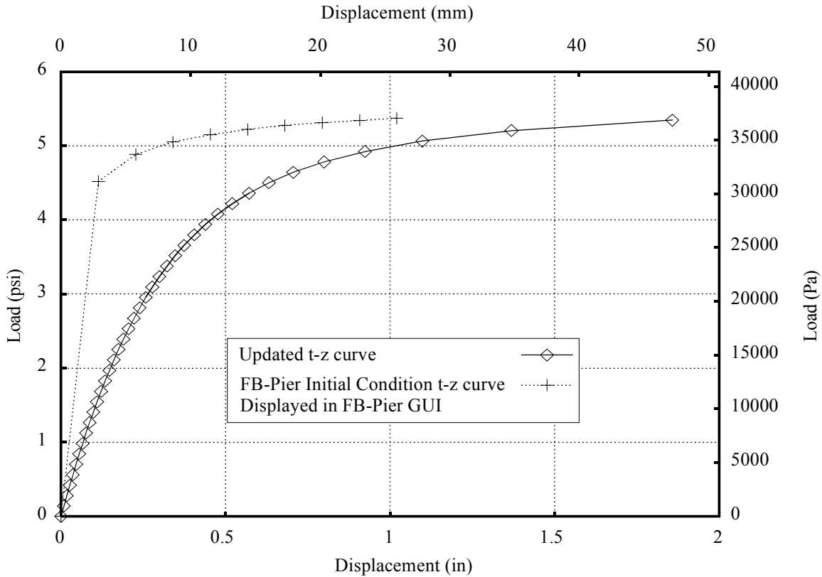
Figure 5.3. TZ-Curve Comparison
