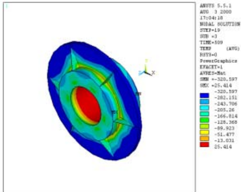
Figure 4.5e Temperature (°F) plot when the lowest critical crack length during AP1 is observed.
