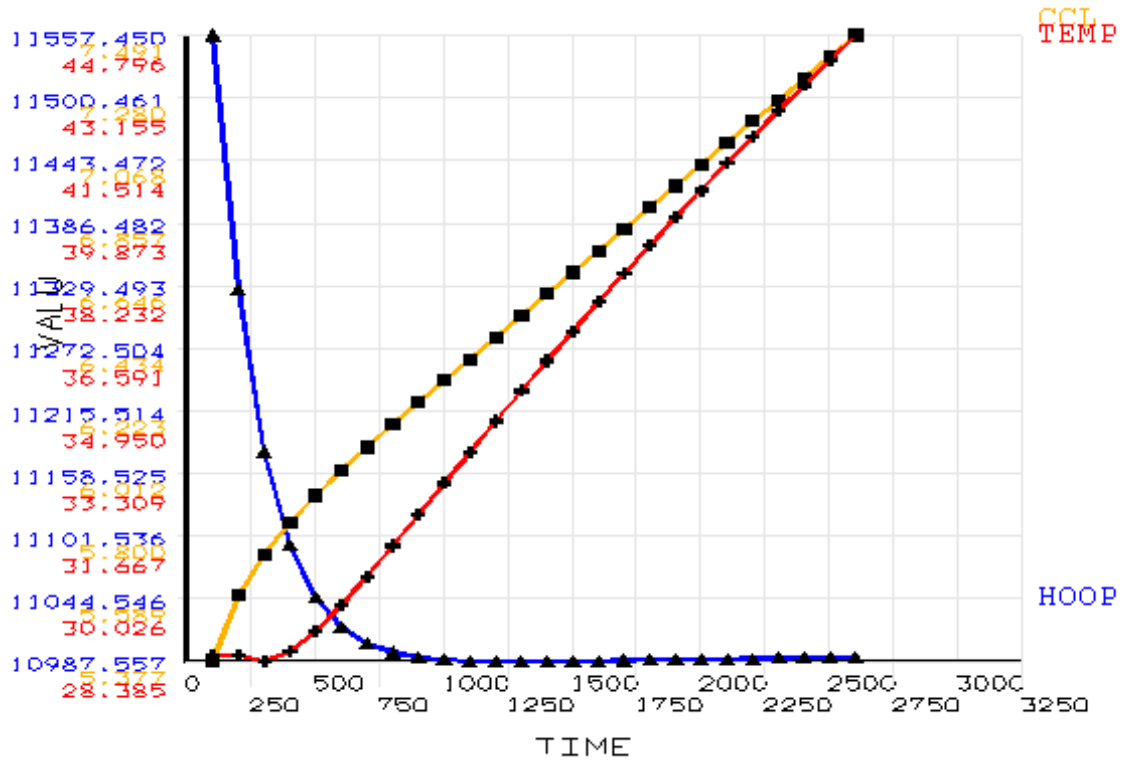
Figure 4.13 Critical parameters (CCL is critical crack length in inches, TEMP is temperature in 0 F, and HOOP is hoop stress in psi) plotted against time (sliding the trunnion into the hub during AP1 of the Hillsborough Avenue Bridge).
