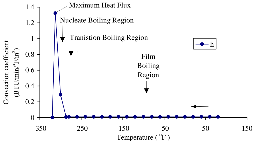
Figure 6.6 Variation of heat transfer coefficient with temperature.
