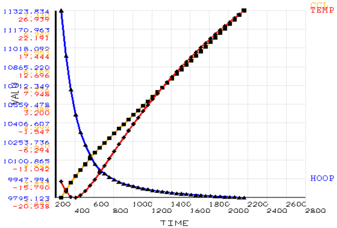
Figure 4.10 Critical parameters (CCL is critical crack length in inches, TEMP is temperature in °F, and HOOP is hoop stress in psi) plotted against time (sliding the trunnion into the hub-girder assembly during AP2 of the Christa McAuliffe Bridge).
