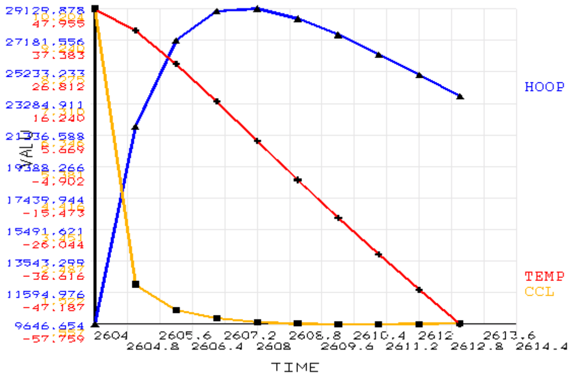
Figure 4.14 Critical parameters (CCL is critical crack length in inches, TEMP is temperature in 0 F, and HOOP is hoop stress in psi) plotted against time (cooling down of the trunnion-hub during AP1 of the Hillsborough Avenue Bridge).
