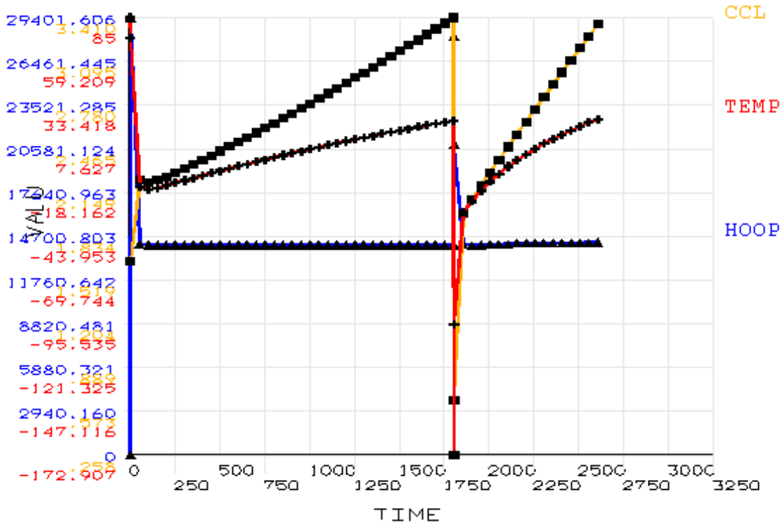
Figure 4.21 Critical parameters (CCL is critical crack length in inches, TEMP is temperature in ^{\circ} F, and HOOP is hoop stress in psi) plotted against time (full assembly process during AP1 of 17 th Street Causeway Bridge).
