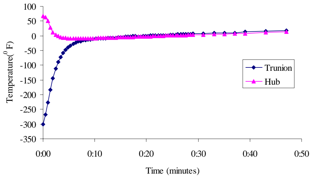
Figure 6.11 Trunnion and hub temperatures during trunnion warm up into the hub.
