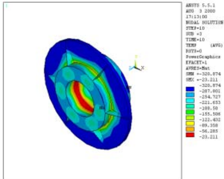
Figure 4.8c Temperature ( ^{\circ} F) plot when the highest hoop stress during AP2 is observed.
