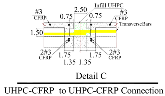
Figure 2.47 Detail of Connections
