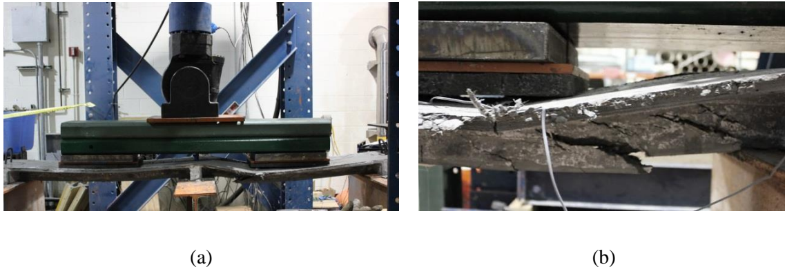
Figure 3.16 Failure Mode of Specimen 1T2S: (a) Deflected Shape, and (b) Shear Crack
