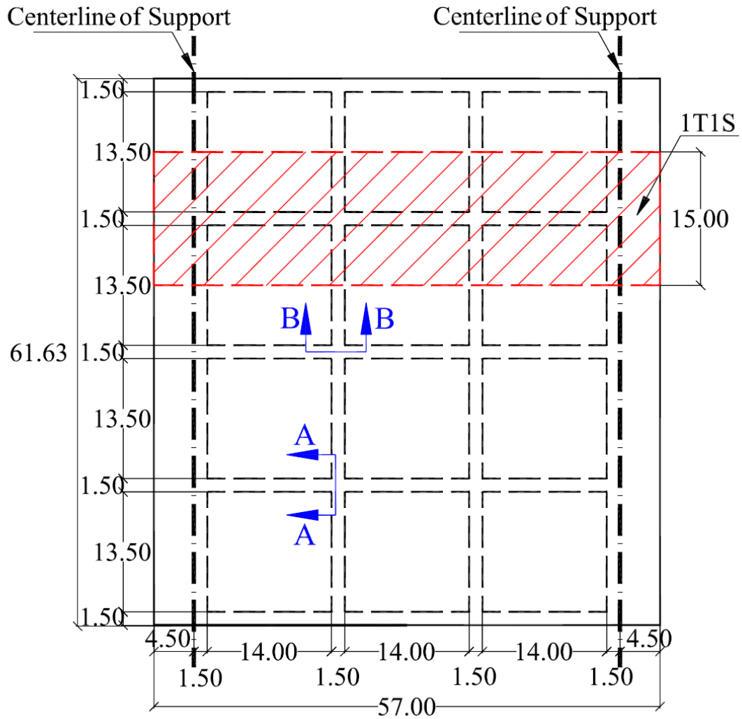
Plan View
