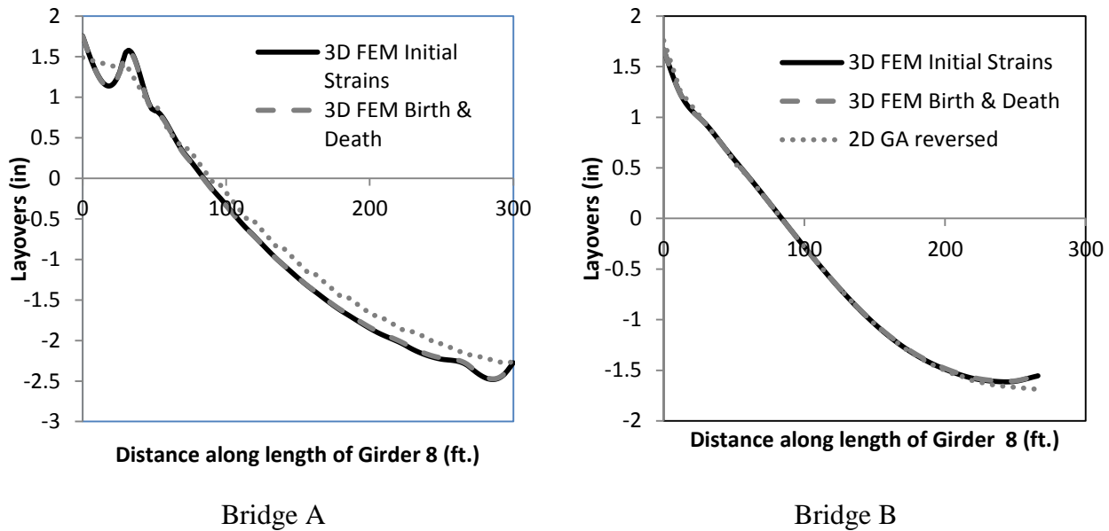
Figure 3.19. Comparison of layovers calculated by different analysis methods—final fit at the SDL stage.
