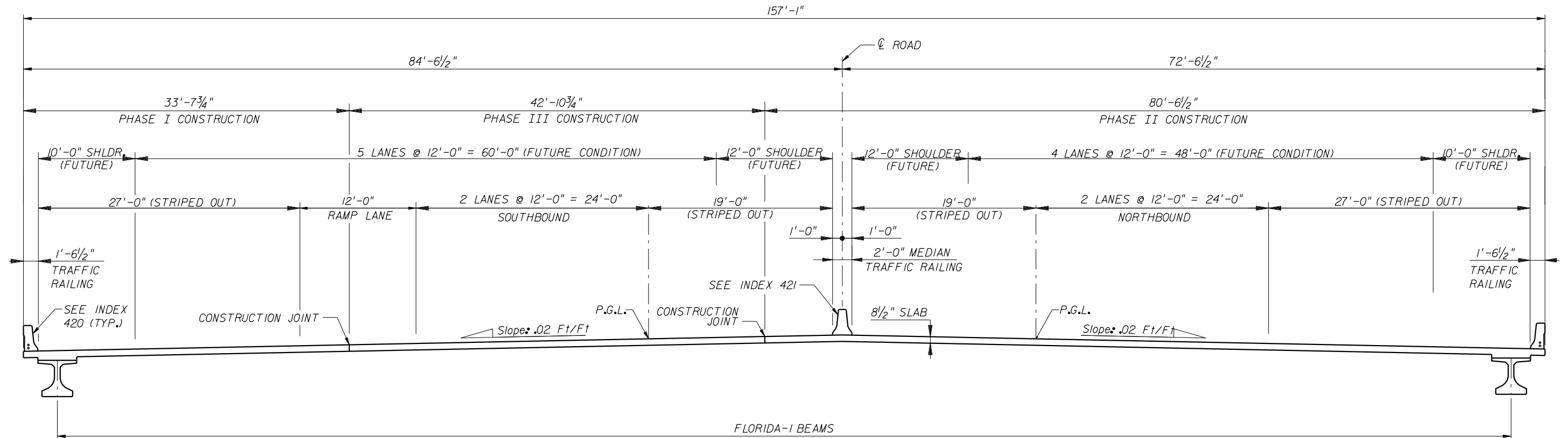
TYPICAL SUPERSTRUCTURE SECTION
