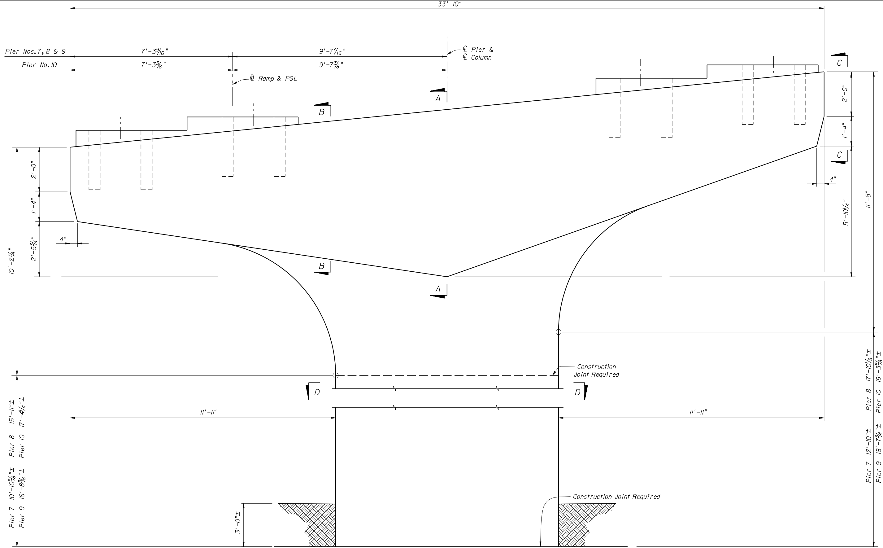
ELEVATION VIEW (Rustication not shown for clarity)
