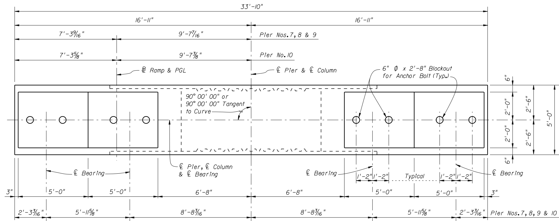
PLAN VIEW PIER NOS. 7, 8, 9 & 10
