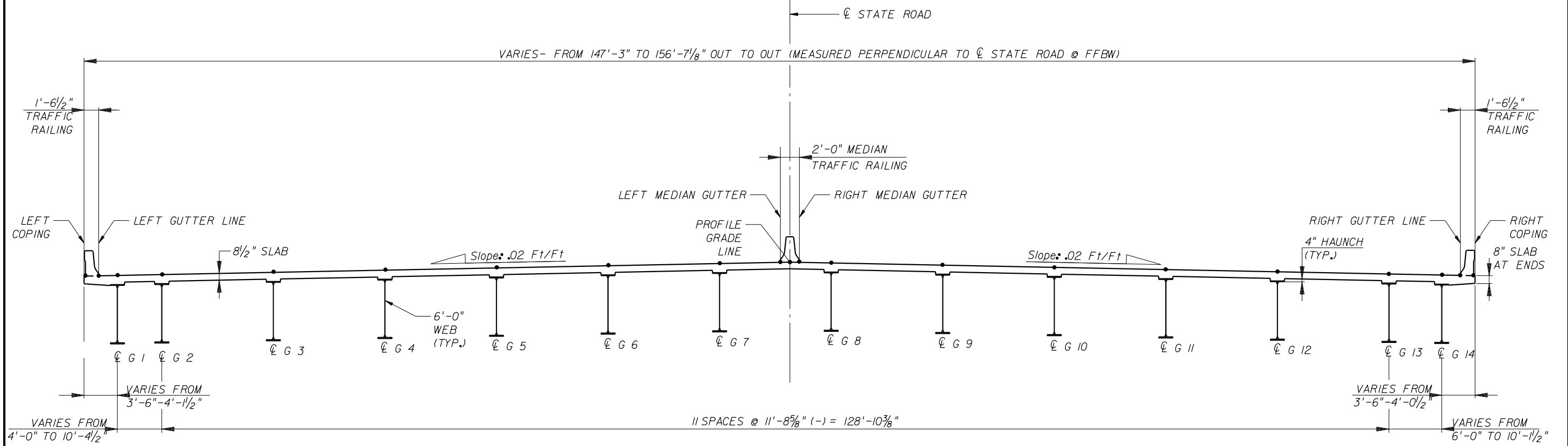
TYPICAL SECTION (LOOKING AHEAD STATION)
