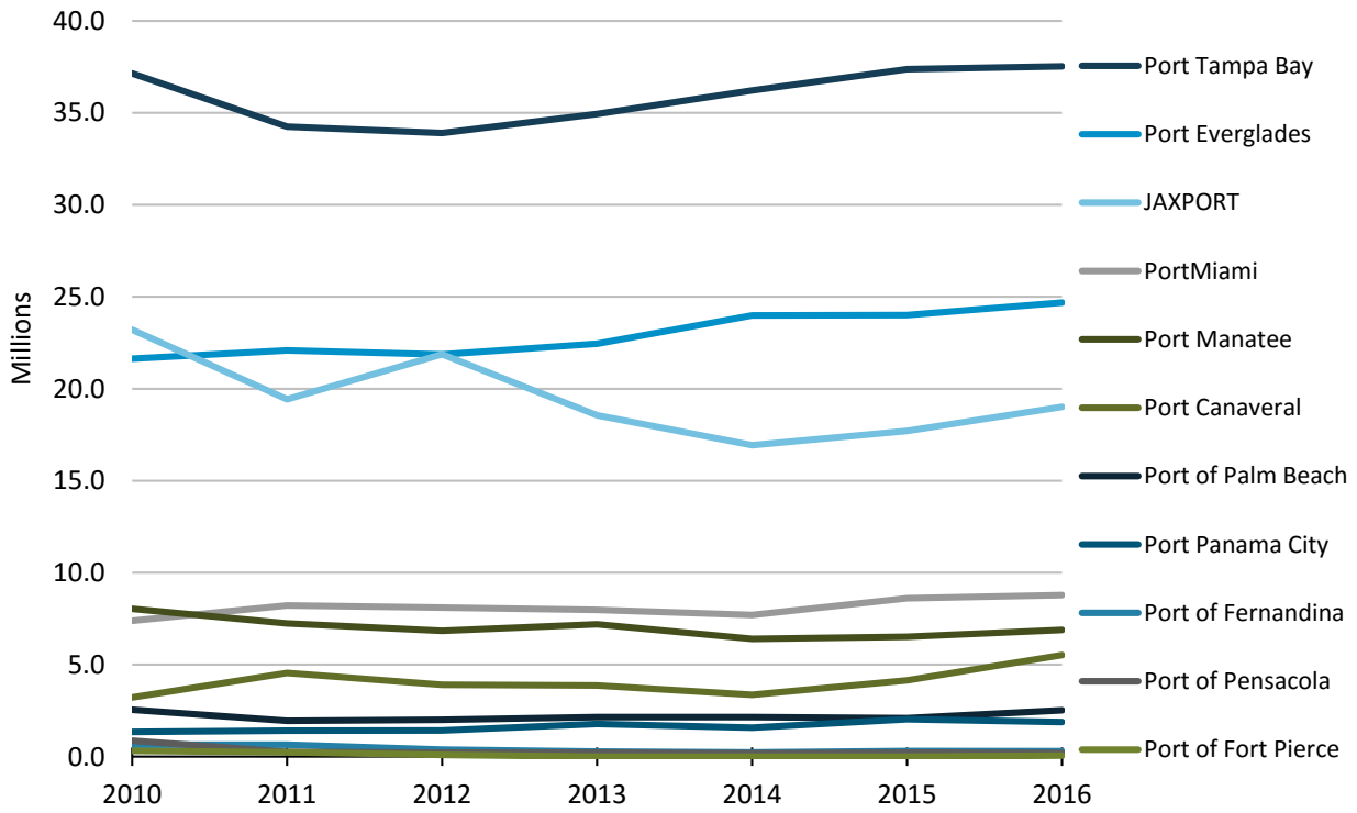
Figure 3-2: Waterborne Tonnage at Florida Seaports (2010 to 2016)
