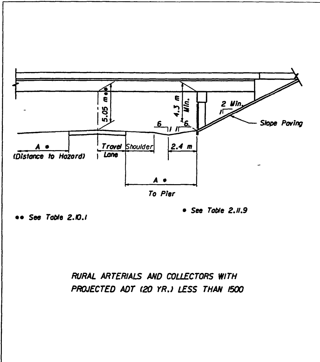
Figure 2.10.2 Clearances
