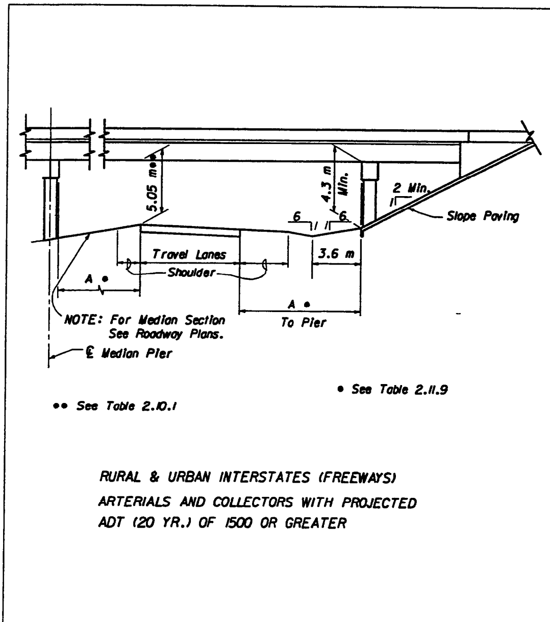
Figure 2.10.1 Clearances
