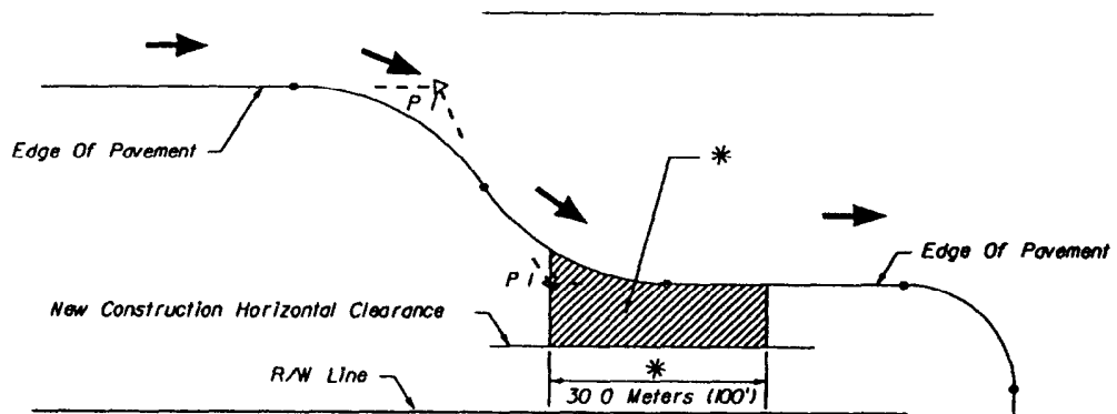
Deceleration For Right Turn With Reverse Curves
