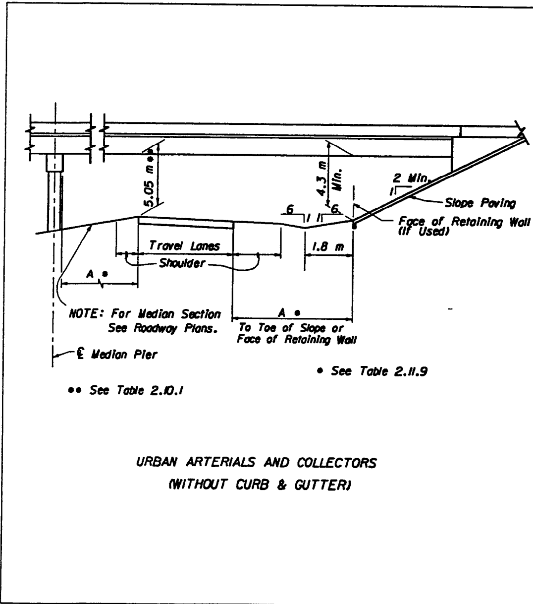
Figure 2.10.3 Clearances
