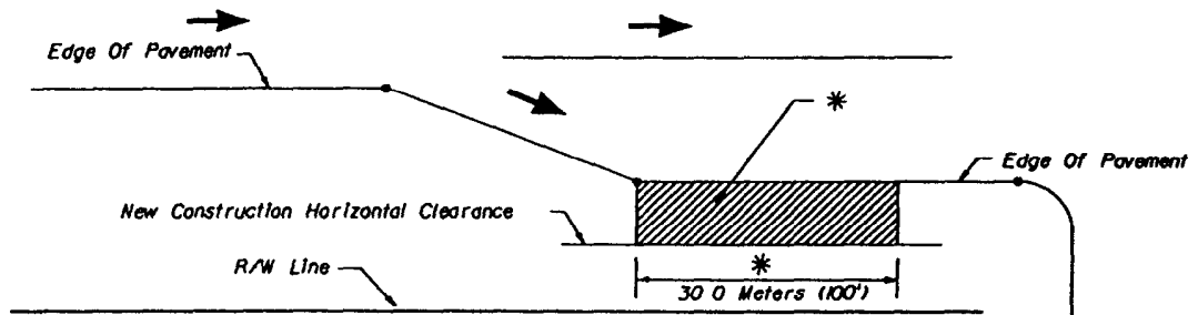
Deceleration For Right Turn With Tangent
