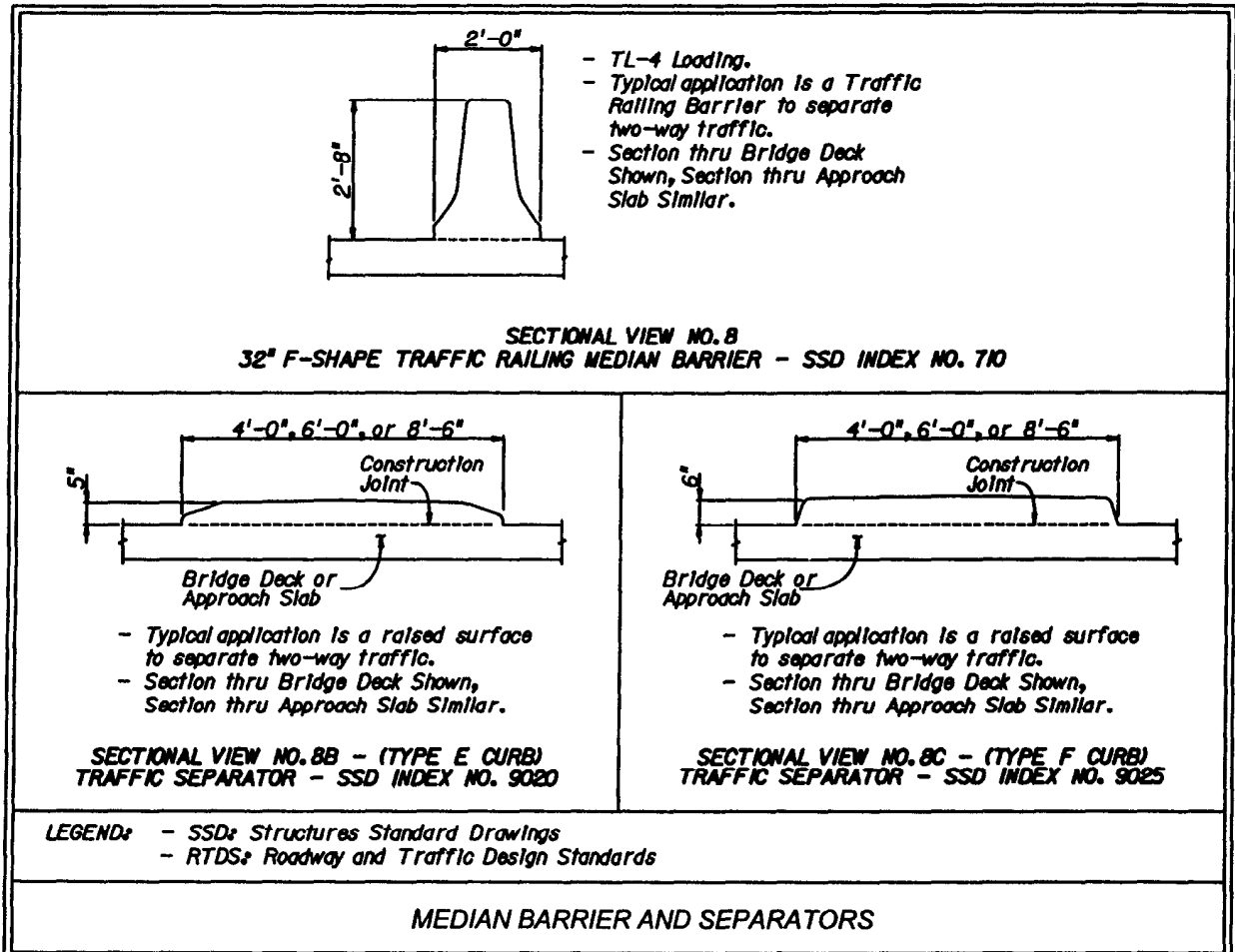
Figure 2.12.4 Bridge Railing and Separators
