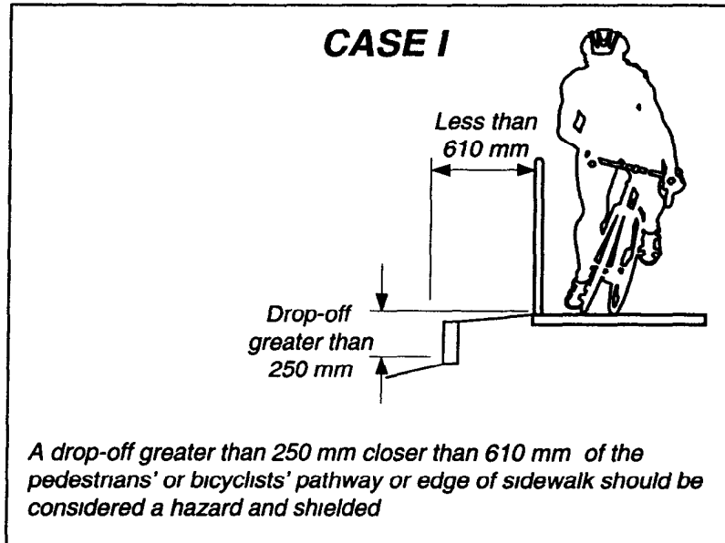
Figure 8.2 Drop-Off Hazards for Pedestrians and Bicyclists
