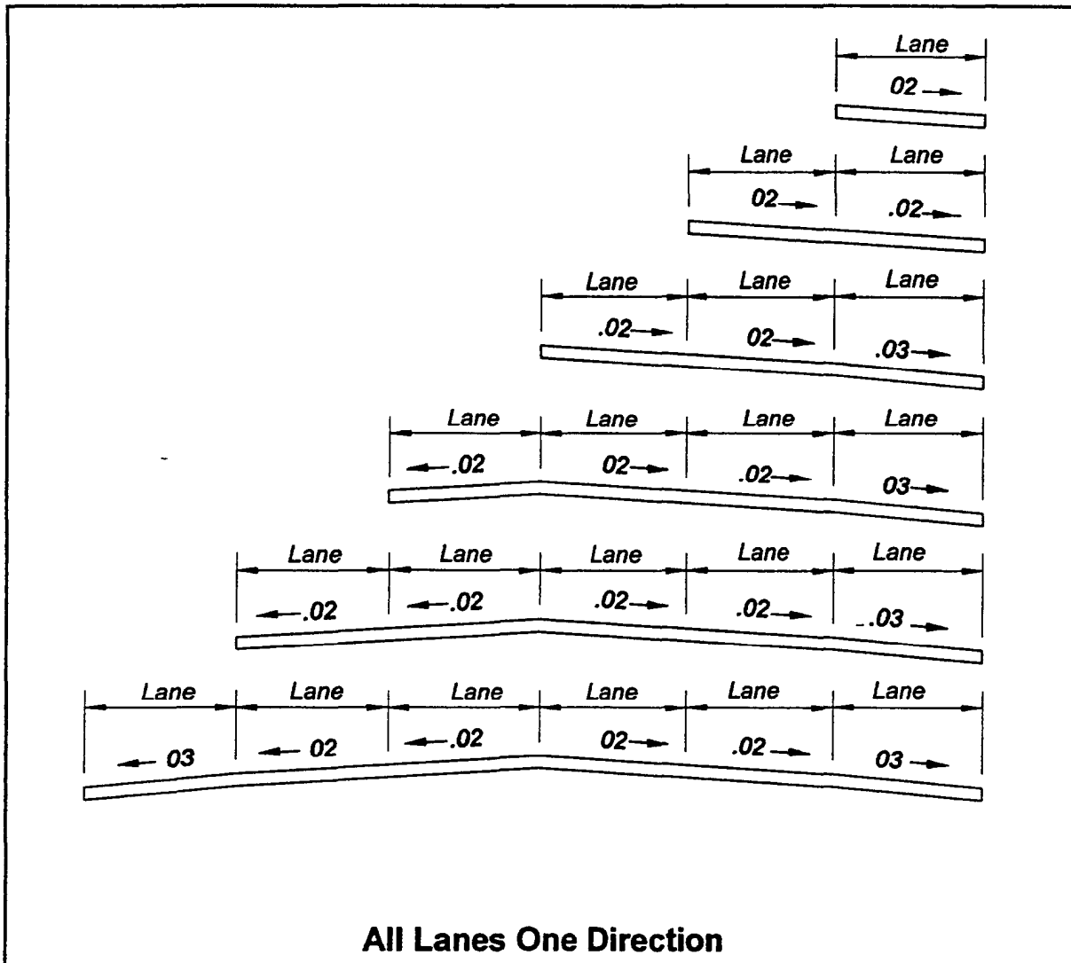
Figure 2.1.1 Standard Pavement Cross Slopes
