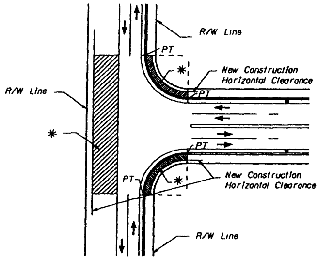
"T" Intersections
