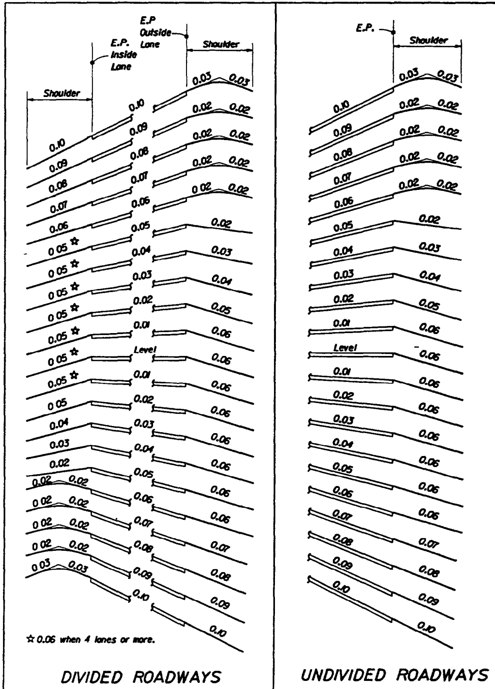
Figure 2.3.1 Shoulder Superelevation
