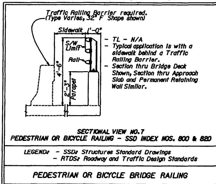
Figure 2.12.3 Bridge Railing
