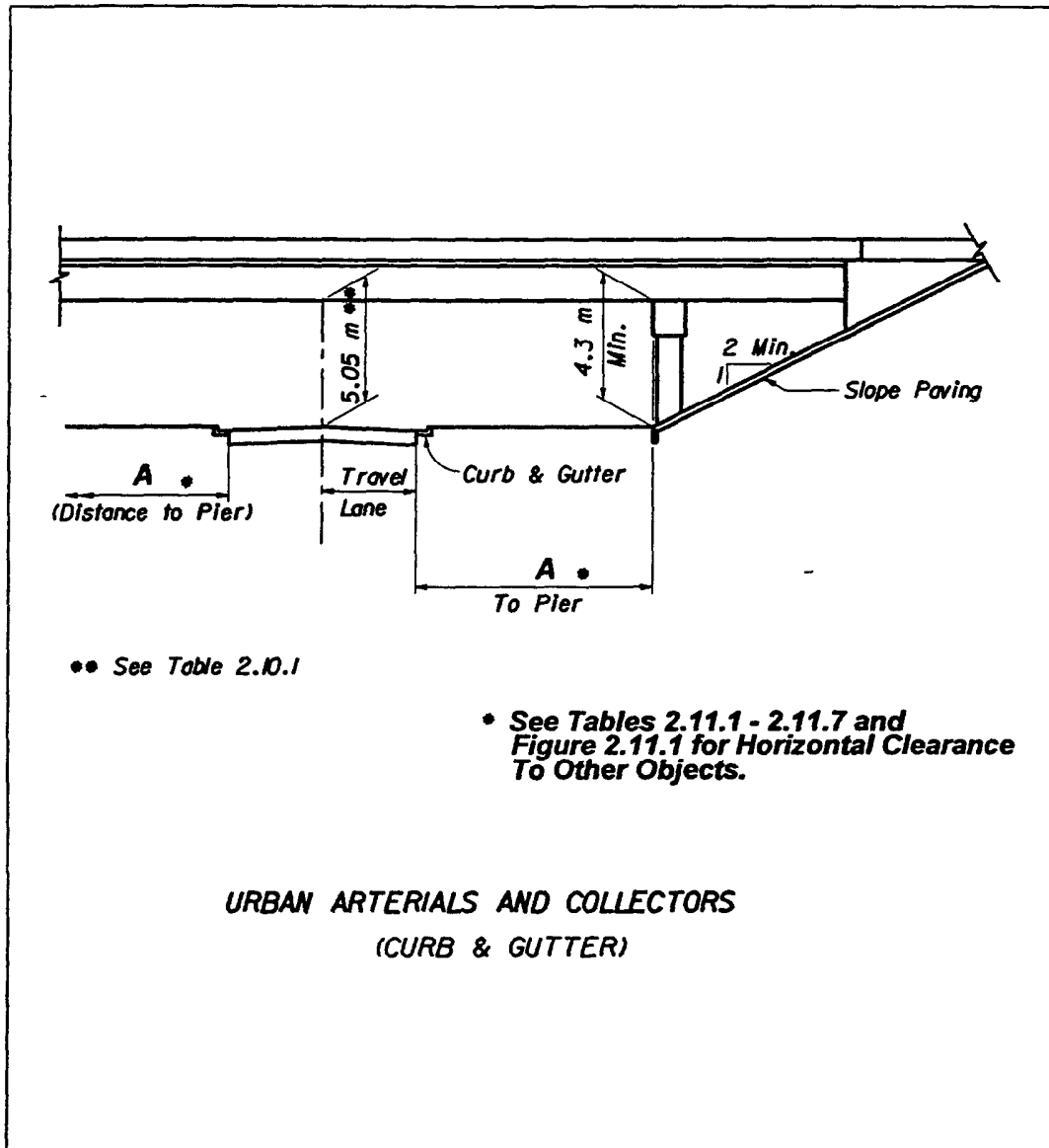
Figure 2.10.4 Clearances
