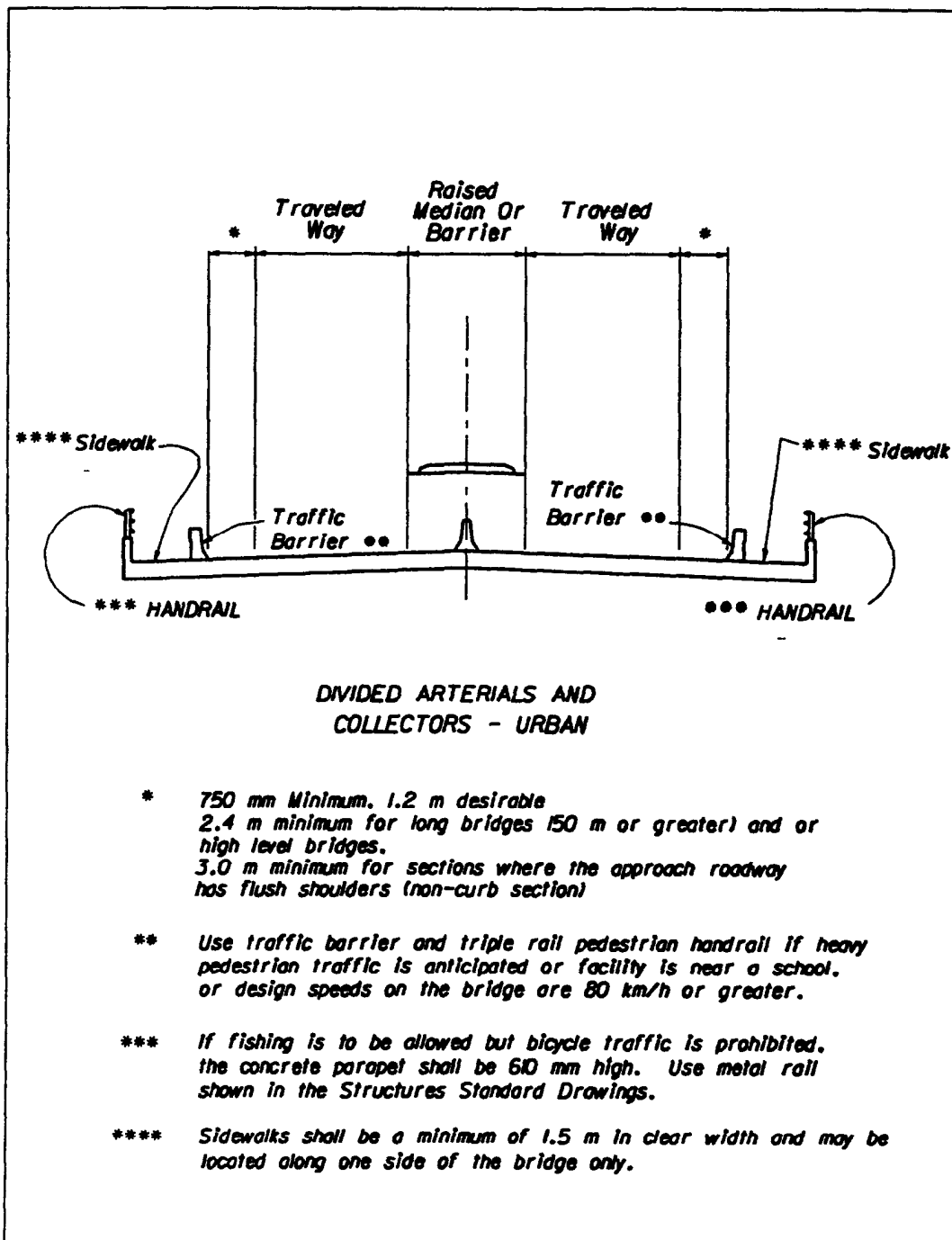
Figure 2.0.4 Bridge Section
