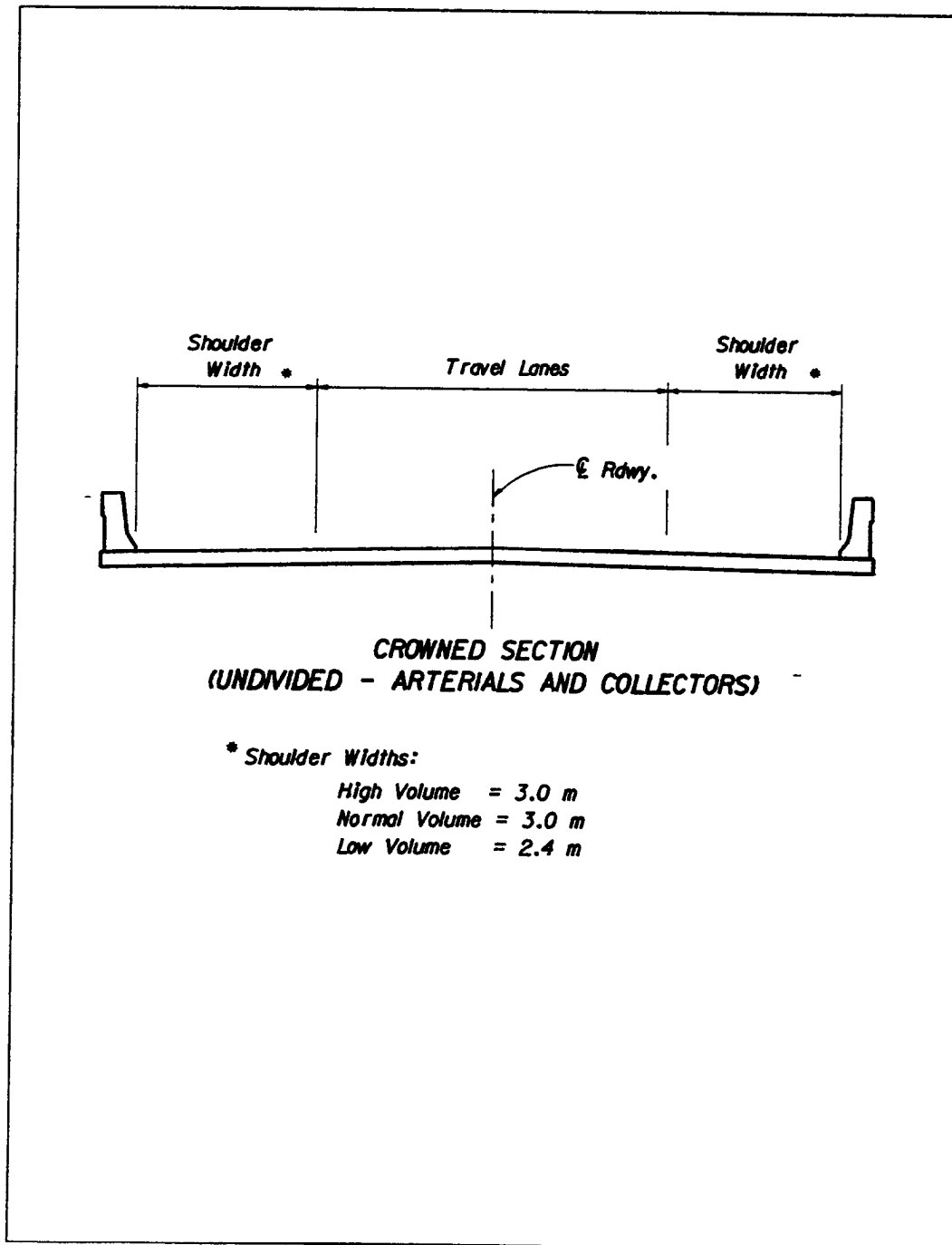
Figure 2.0.2 Bridge Section
