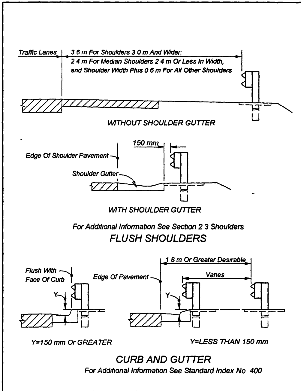
Figure 2.11.1 Horizontal Clearance To Guardrail
