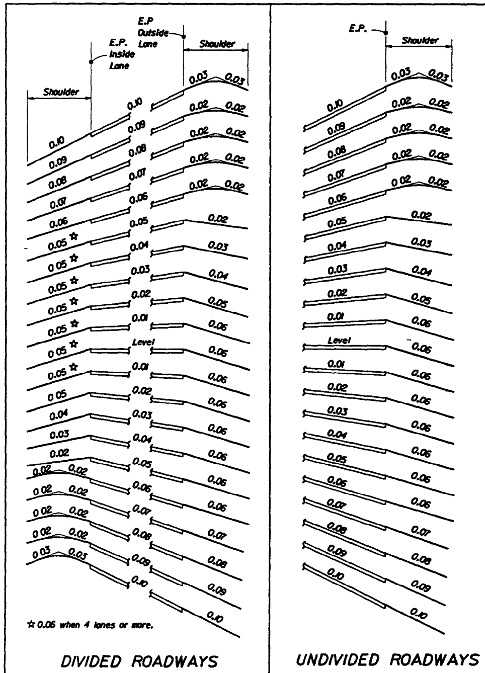
Figure 2.3.1 Shoulder Superelevation
