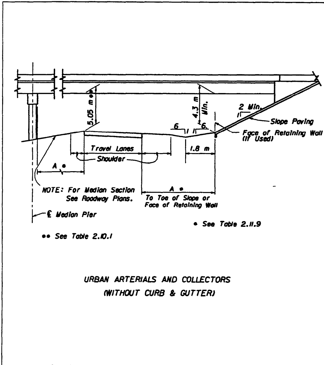
Figure 2.10.3 Clearances
