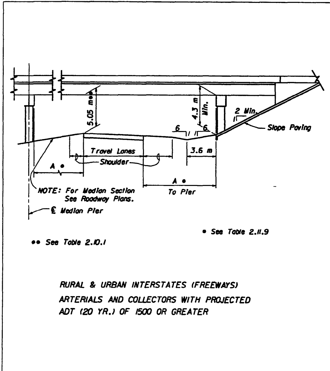
Figure 2.10.1 Clearances
