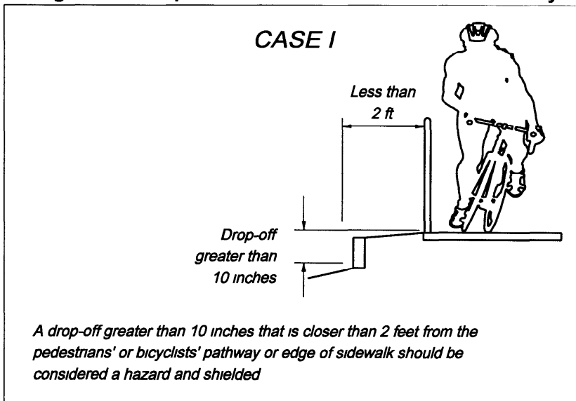
Figure 8 2 Drop-Off Hazards for Pedestrians and Bicyclists
