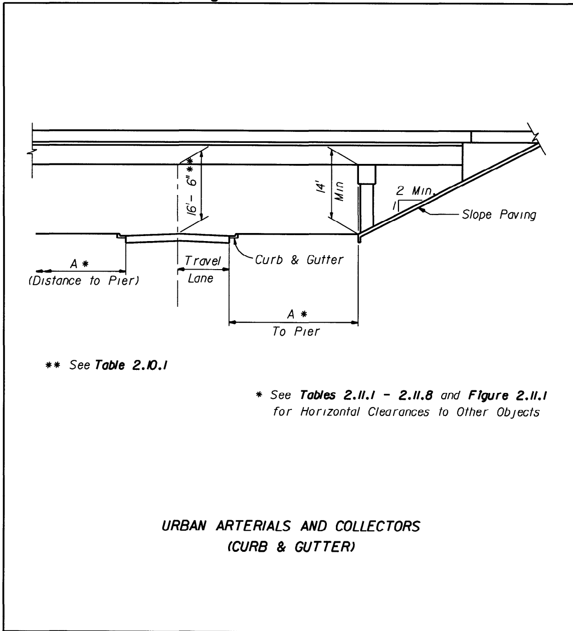
Figure 2 10 4 Clearances
