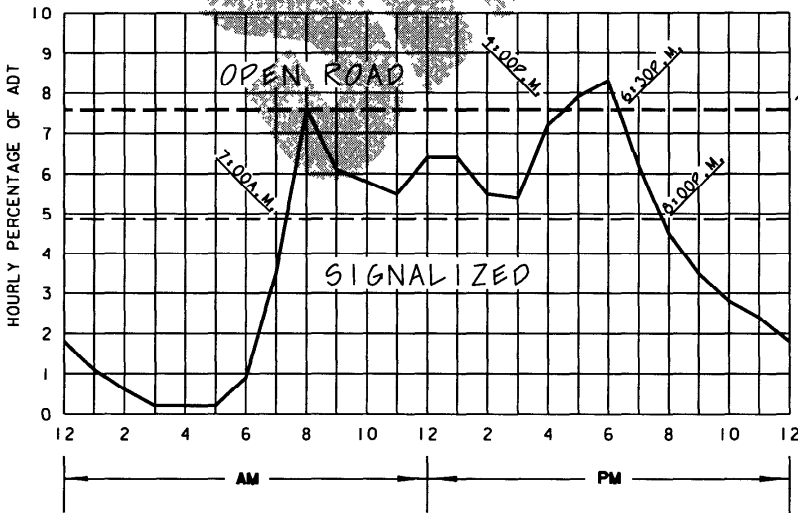
HOURLY VARIATION OF DAILY TRAFFIC
