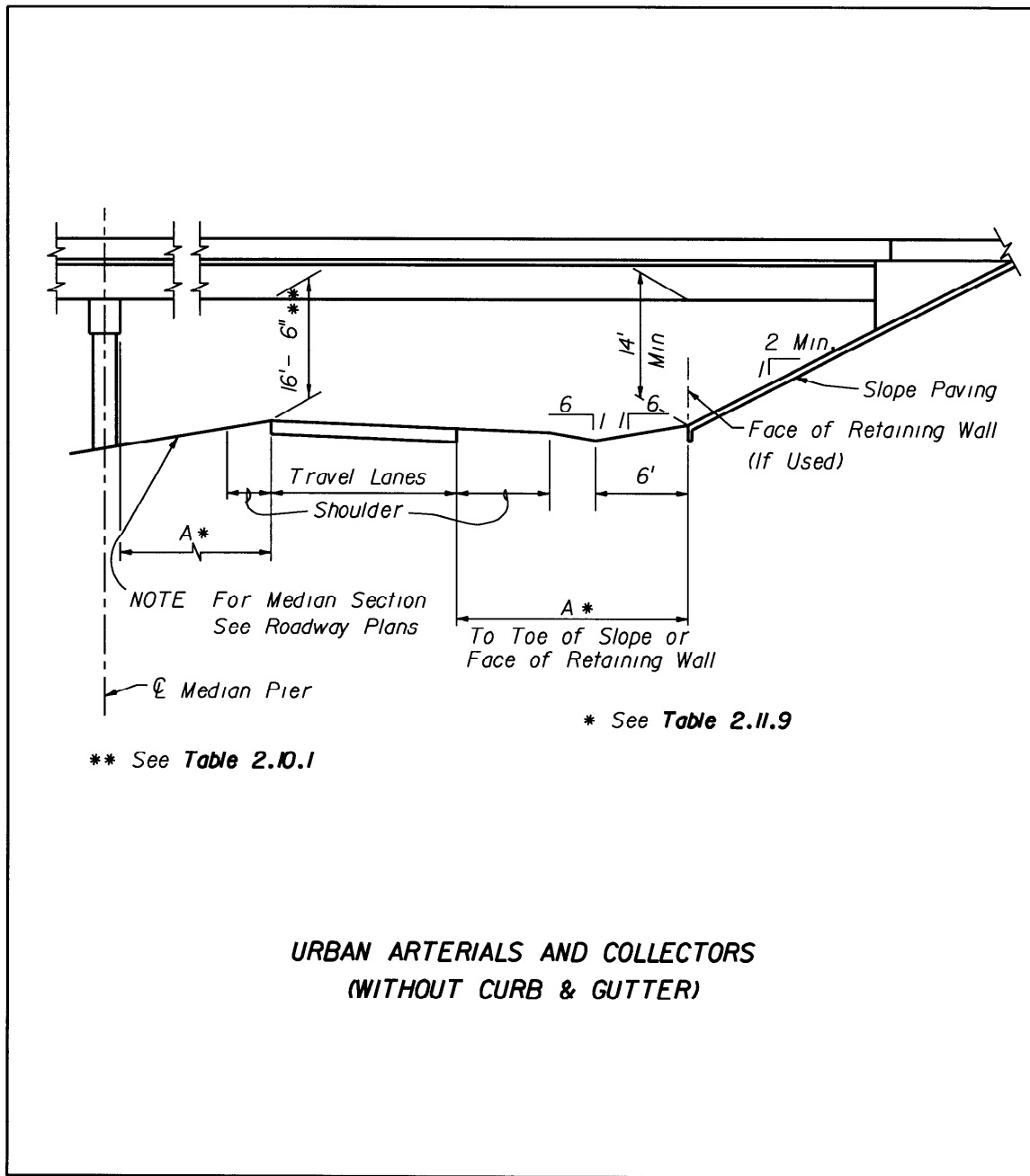
Figure 2 10 3 Clearances
