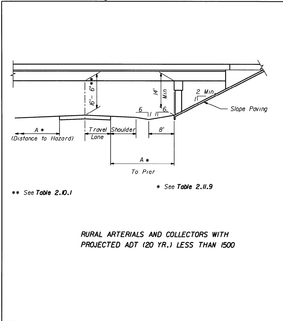
Figure 2 10 2 Clearances
