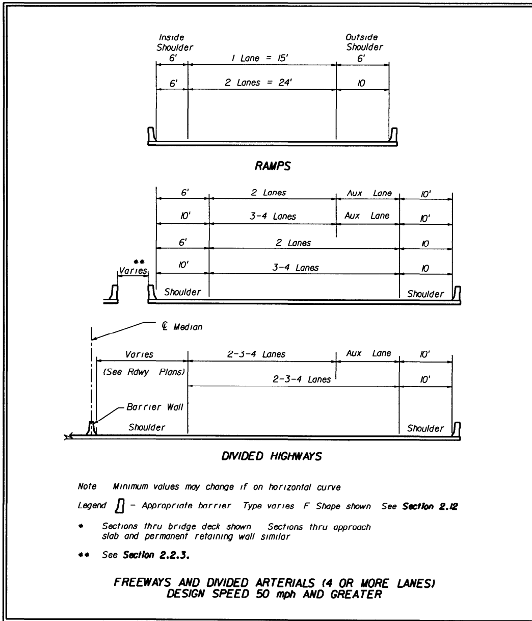
Figure 2 0.1 Partial Bridge Sections *
