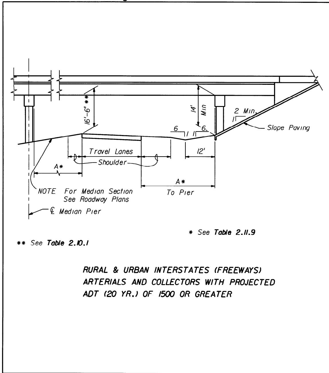
Figure 2 10.1 Clearances
