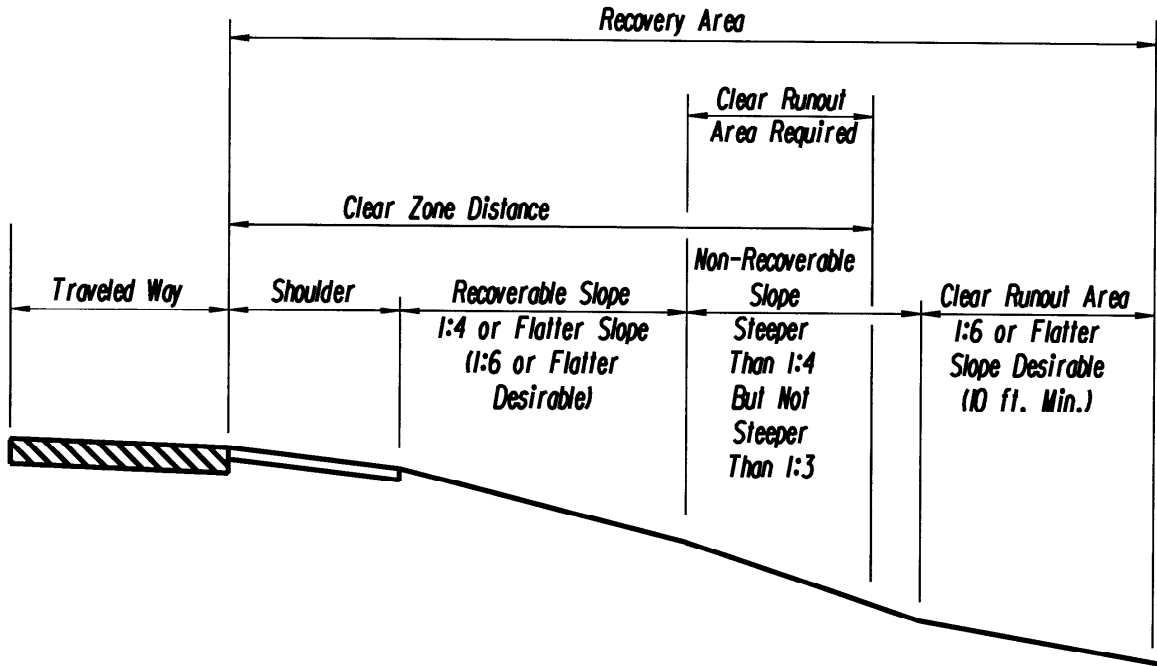
Figure 4 1 2 Recovery Area And Clear Zone Distance
