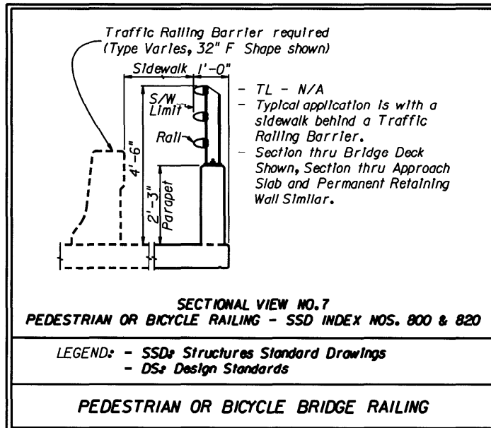
Figure 2.12 3 Bridge Railing
