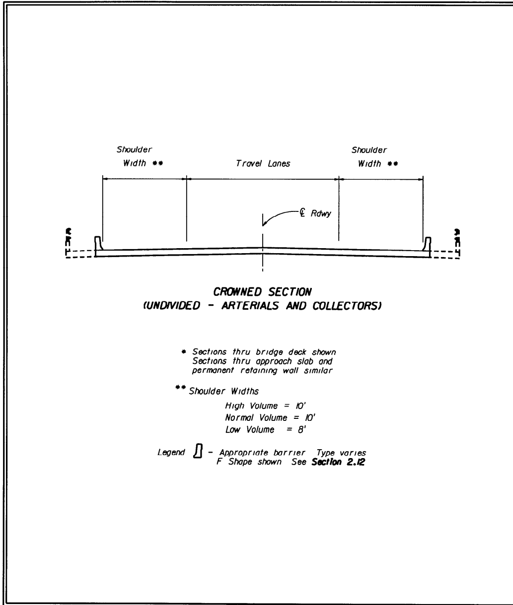
Figure 2.0.2 Bridge Section *
