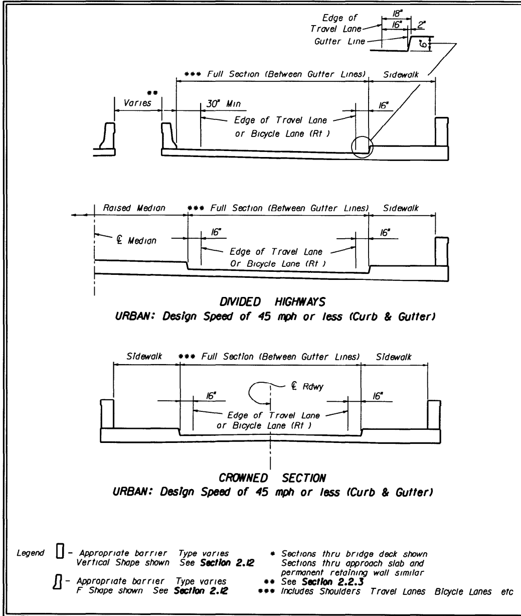
Figure 2 0 3 Partial Bridge Sections *
