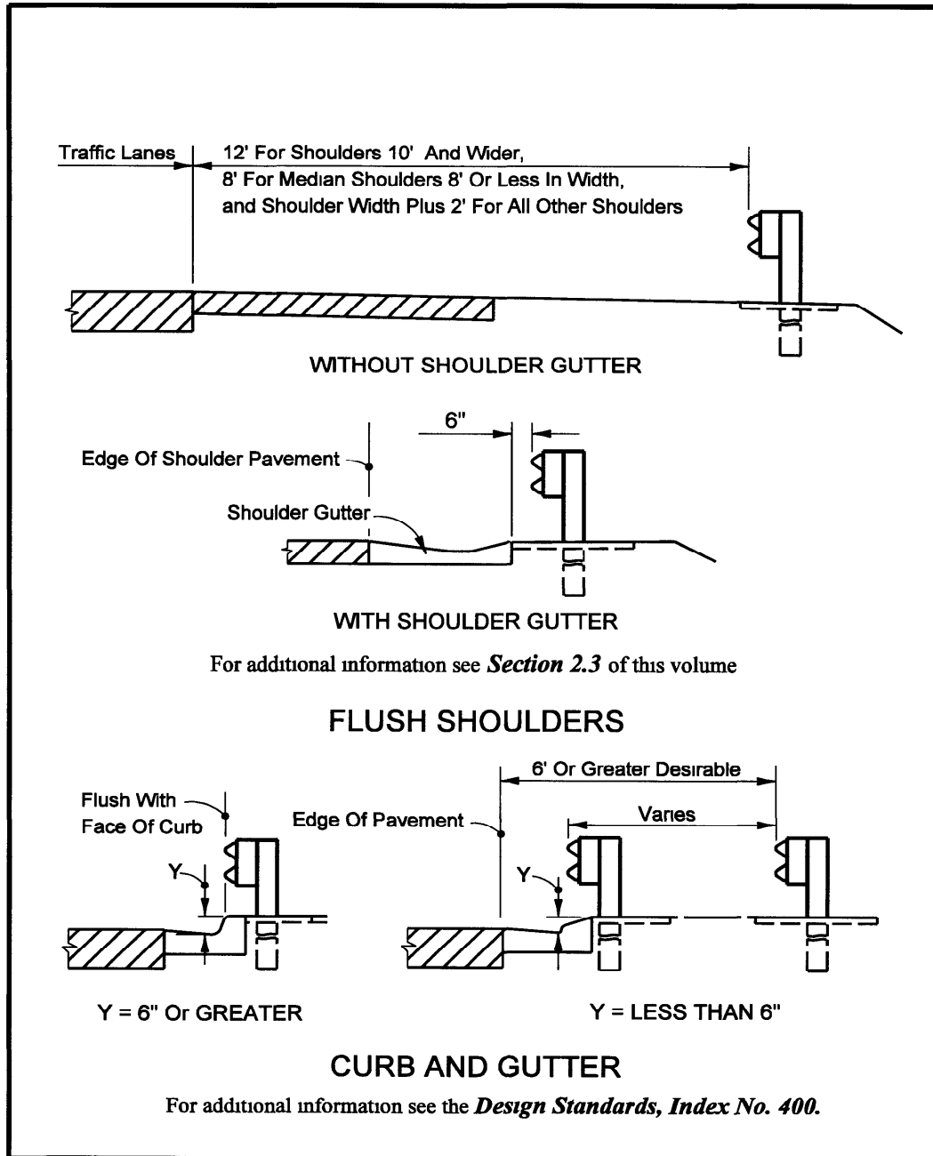
Figure 2 11 1 Clearance to Guardrail
