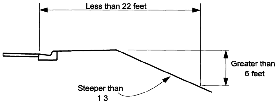
Figure 4.2.2 Drop-off Hazards in Urban Sections
