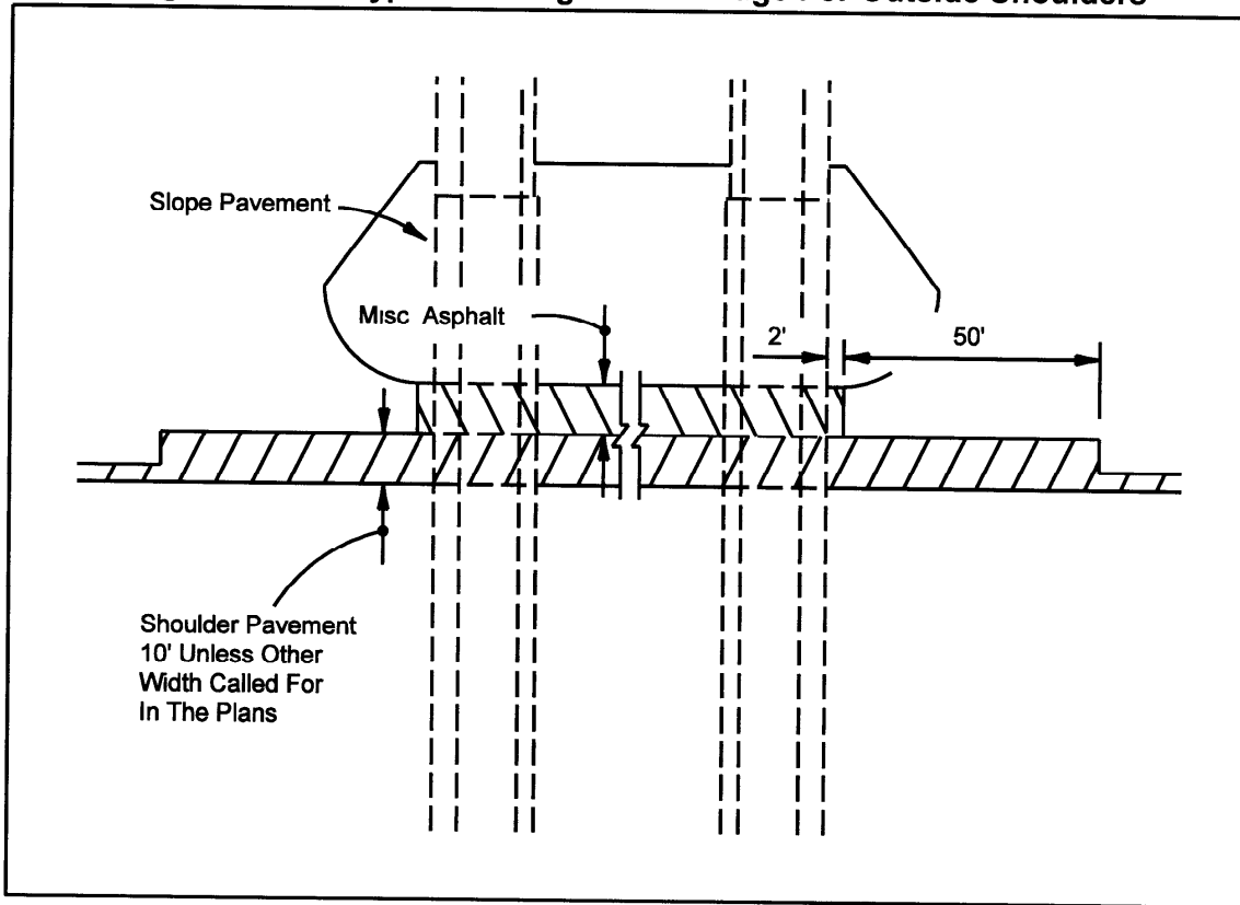
Figure 2 3 2 Typical Paving Under Bridge For Outside Shoulders
