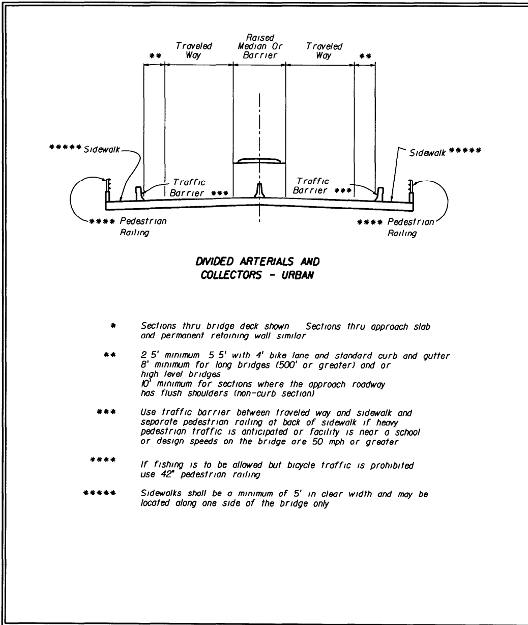
Figure 2 0 4 Bridge Section *
