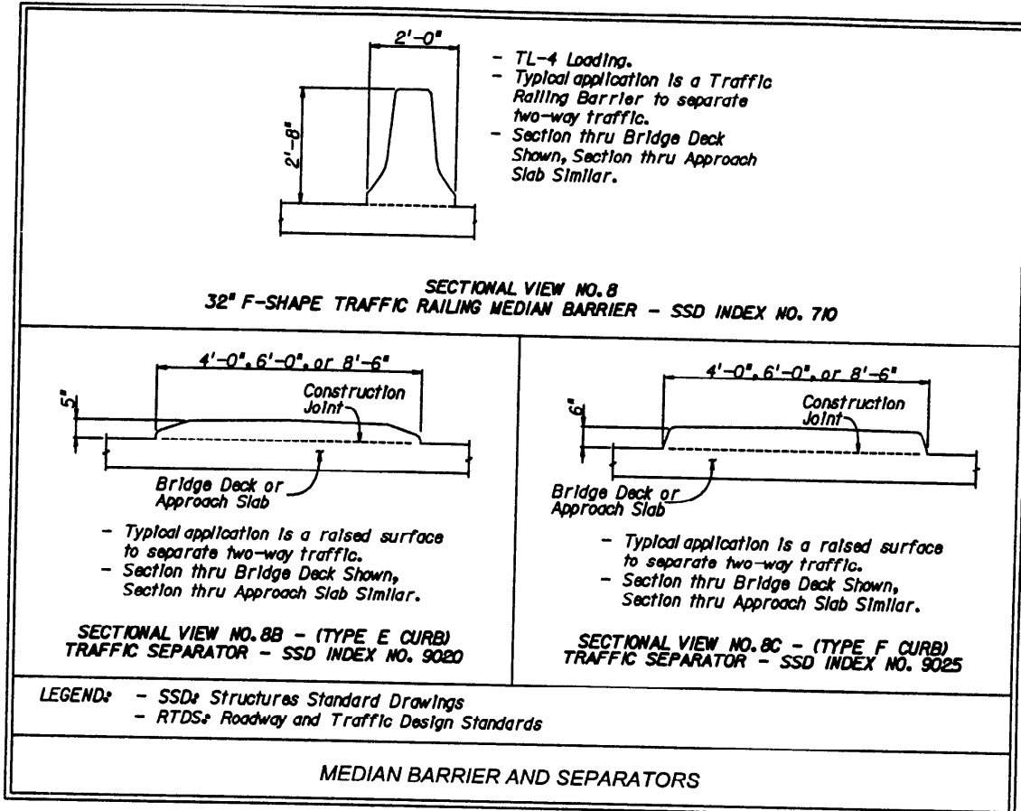
Figure 2.12.4 Bridge Railing and Separators
