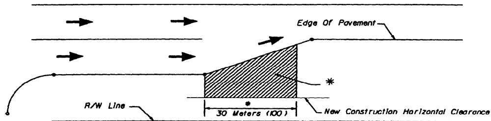
Lane Termination Using A Skewed Merge Section
