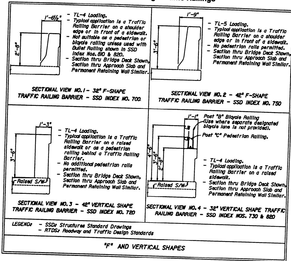
Figure 2.12.1 Bridge Traffic Railings
