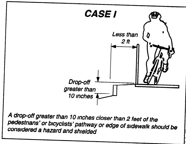
Figure 8.2 Drop-Off Hazards for Pedestrians and Bicyclists
