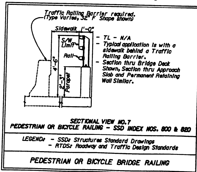
Figure 2.12.3 Bridge Railing
