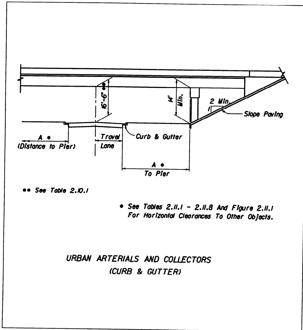
Figure 2.10.4 Clearances
