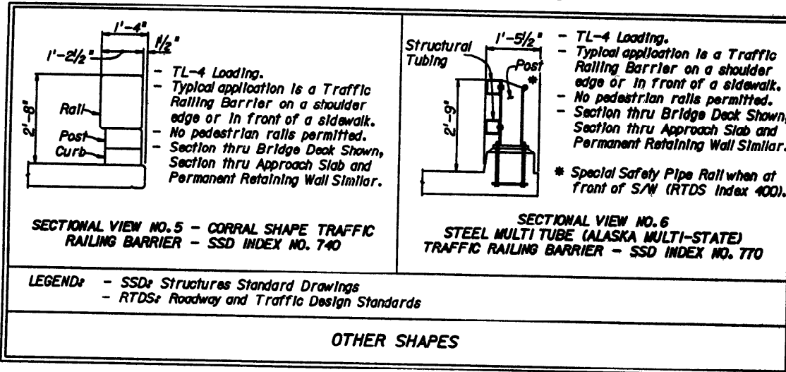
Figure 2.12.2 Bridge Traffic Railings
