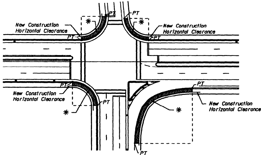
Intersecting Streets
