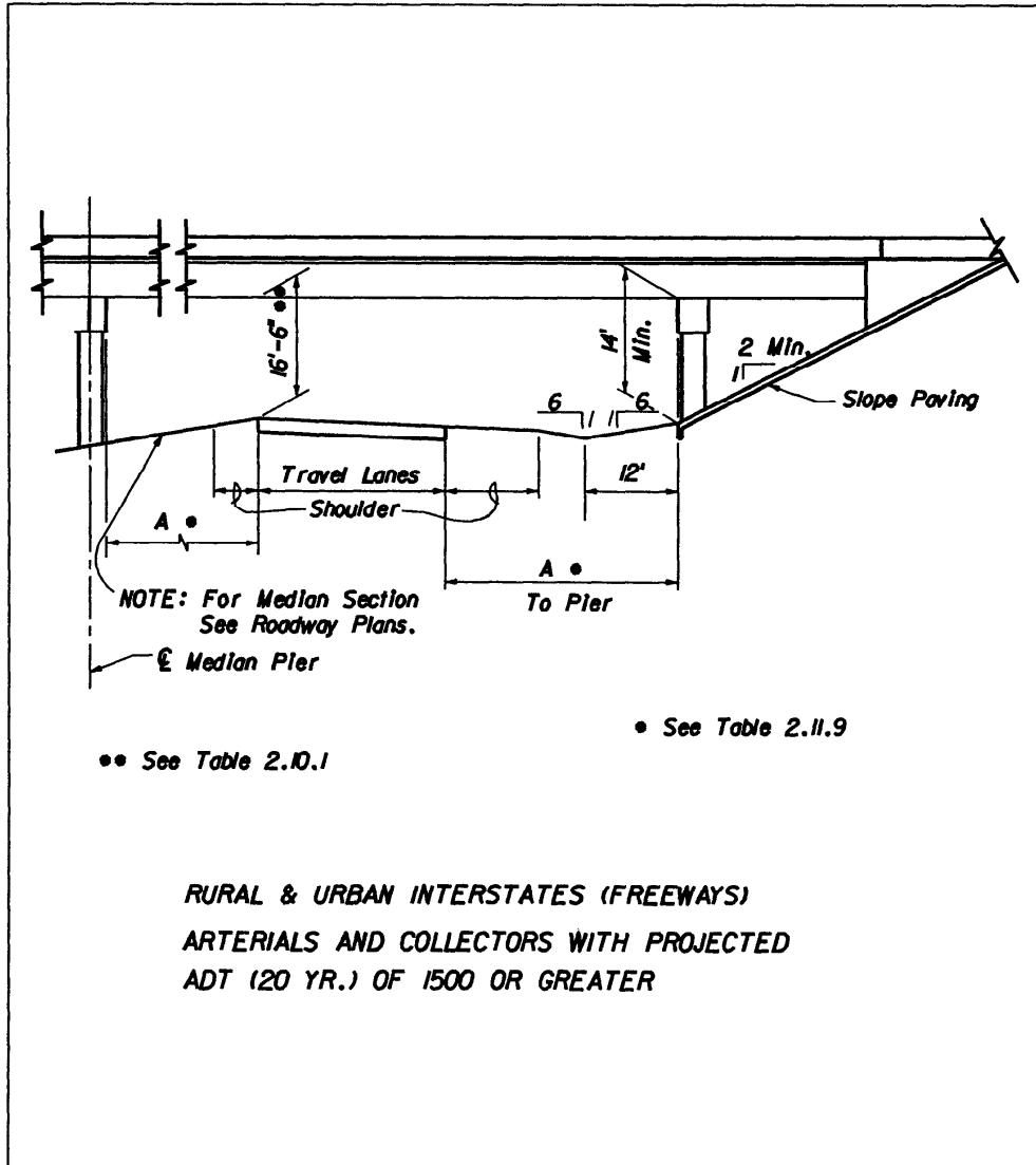
Figure 2.10.1 Clearances
