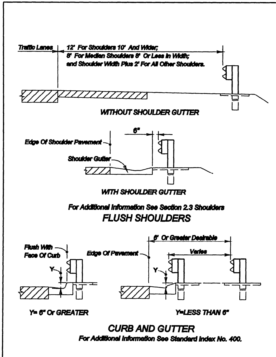
Figure 2.11.1 Clearance to Guardrail
