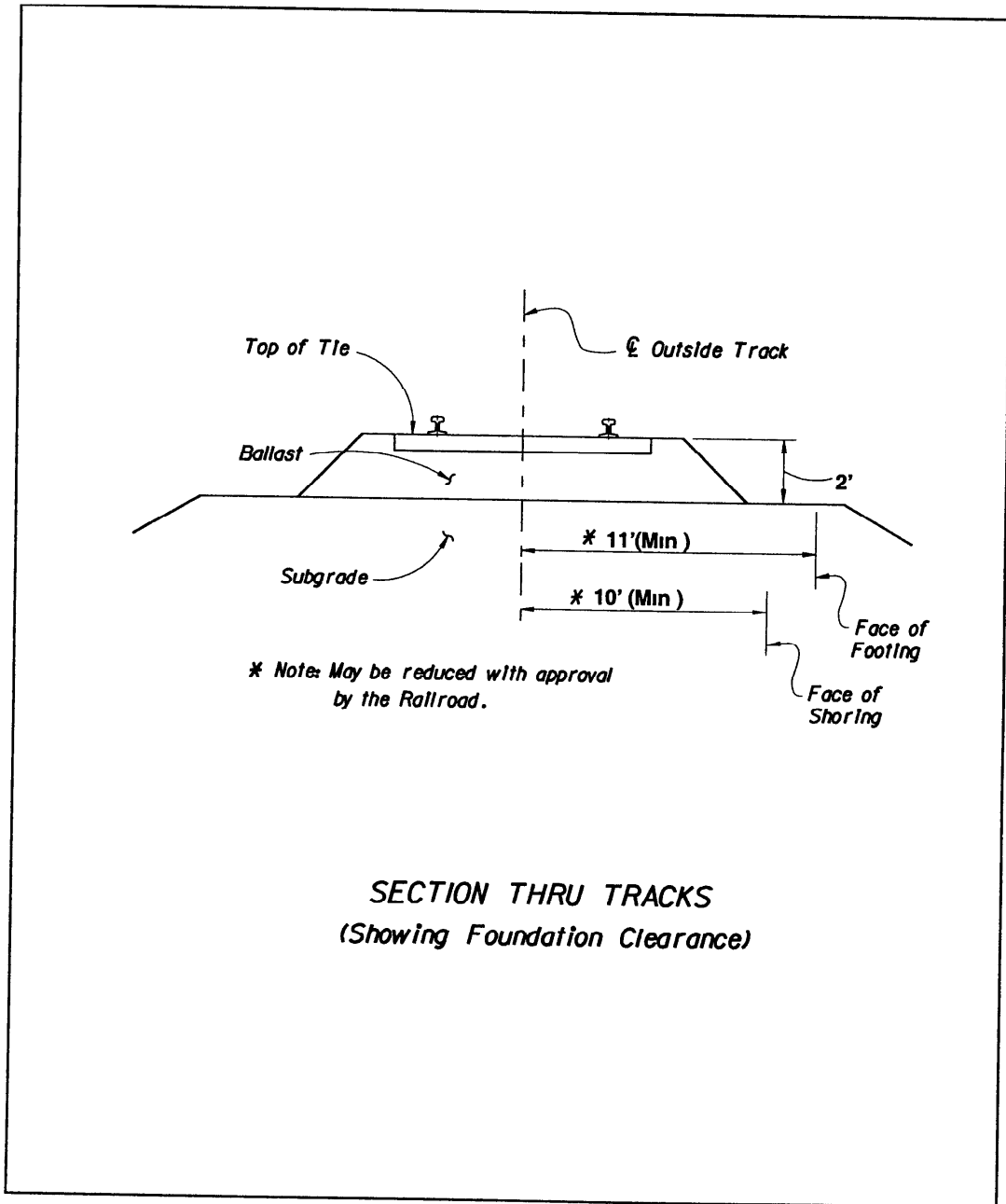
Figure 6.3 Section Thru Tracks
