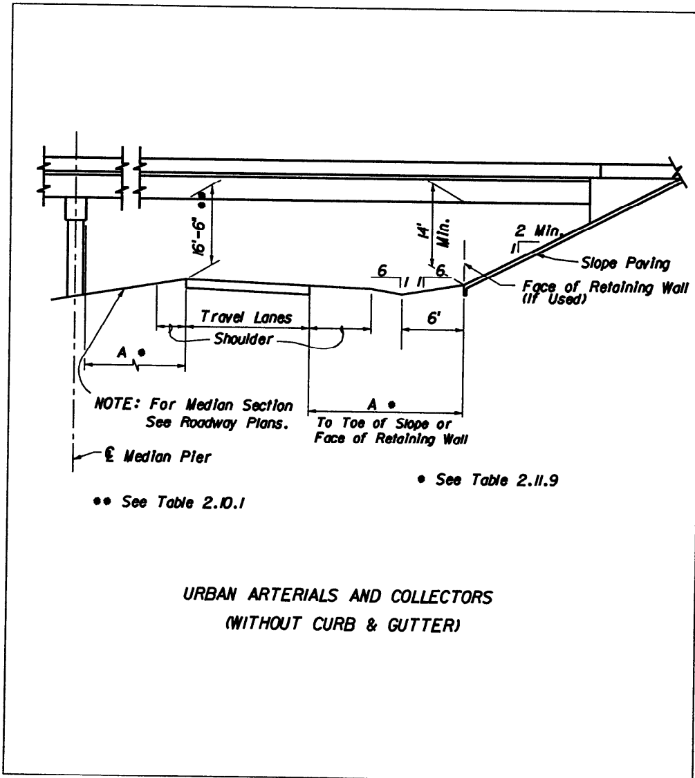
Figure 2.10.3 Clearances
