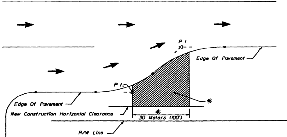
Lane Termination Using A Reverse Curve
