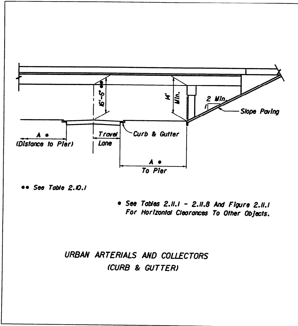
Figure 2 10.4 Clearances
