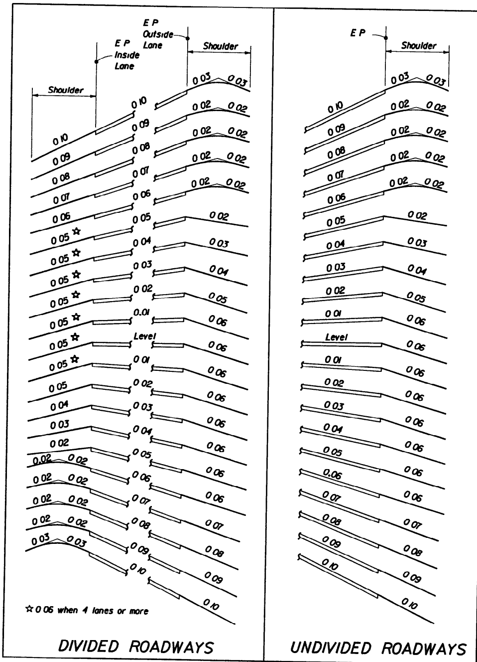
Figure 2.3.1 Shoulder Superelevation
