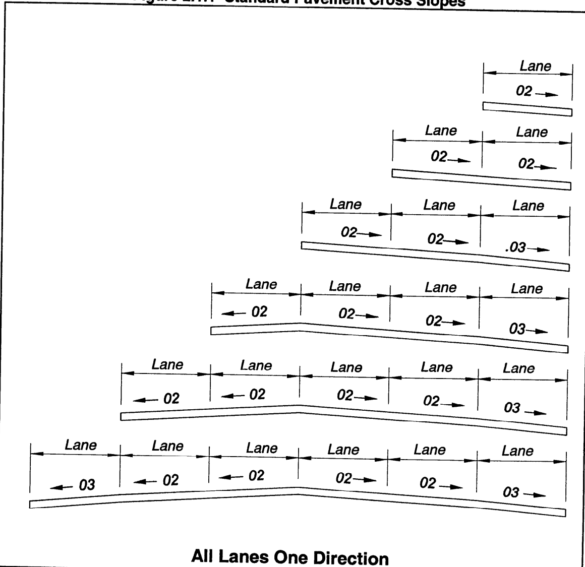
Figure 2.1.1 Standard Pavement Cross Slopes
