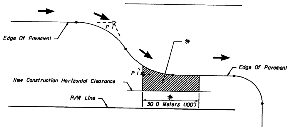
Deceleration For Right Turn With Reverse Curves
