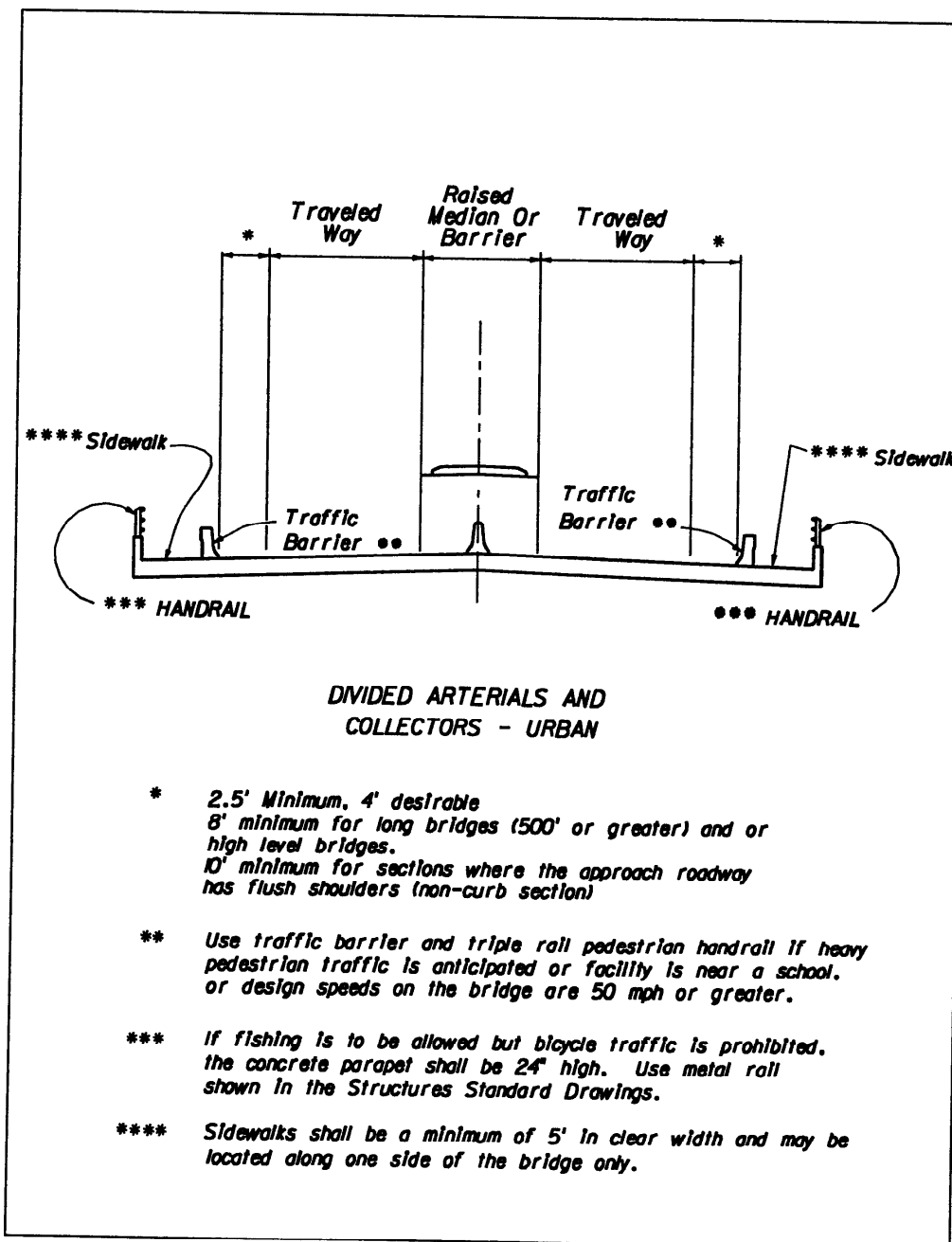
Figure 2.0.4 Bridge Section
