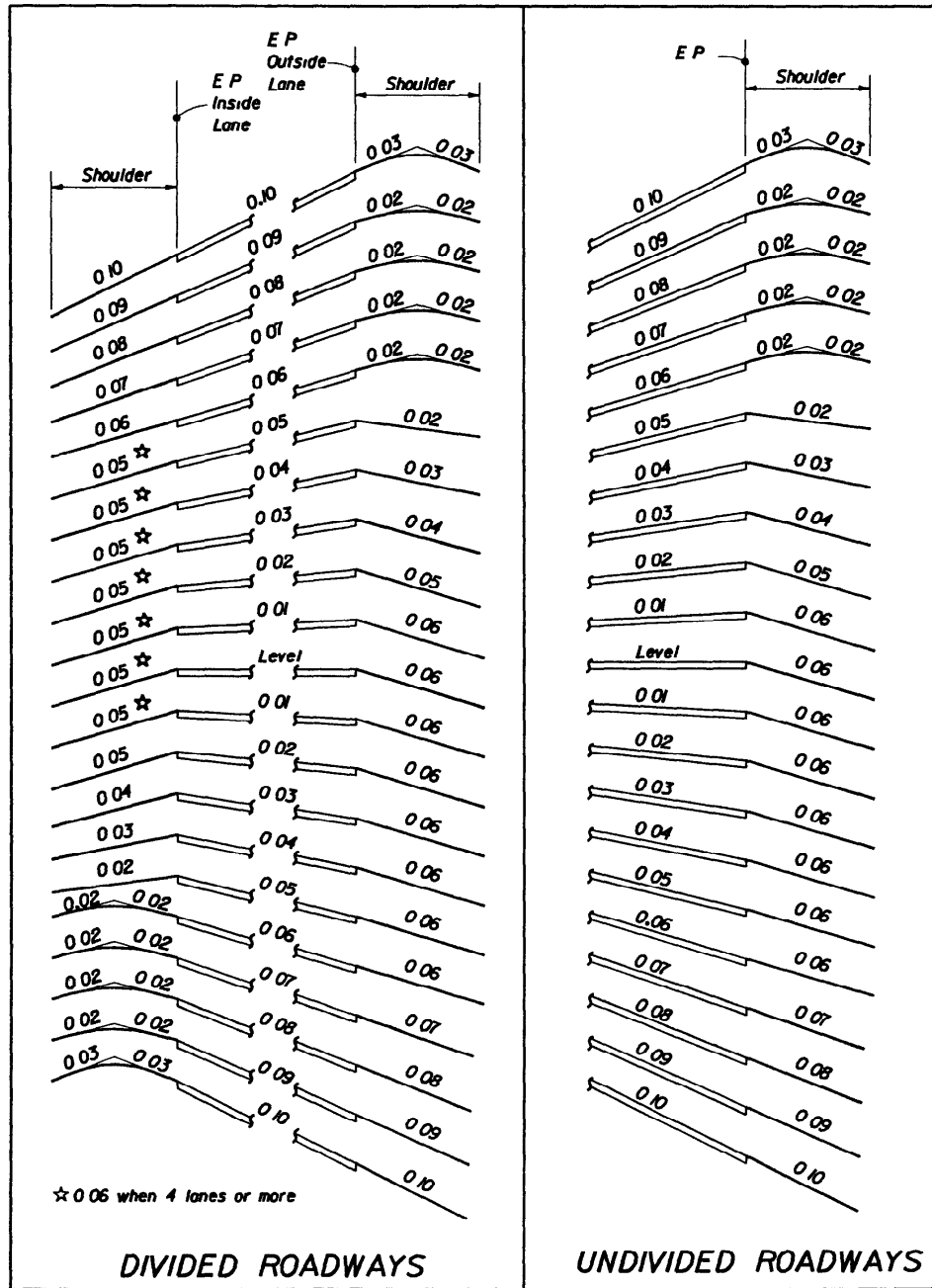
Figure 2.3.1 Shoulder Superelevation
