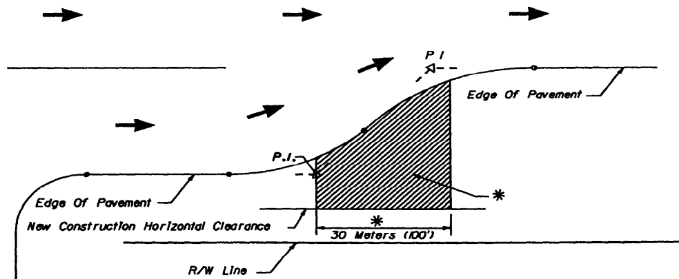
Lane Termination Using A Reverse Curve
