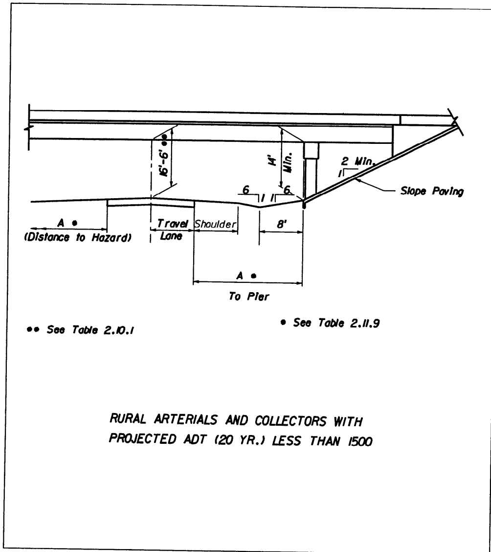
Figure 2 10 2 Clearances
