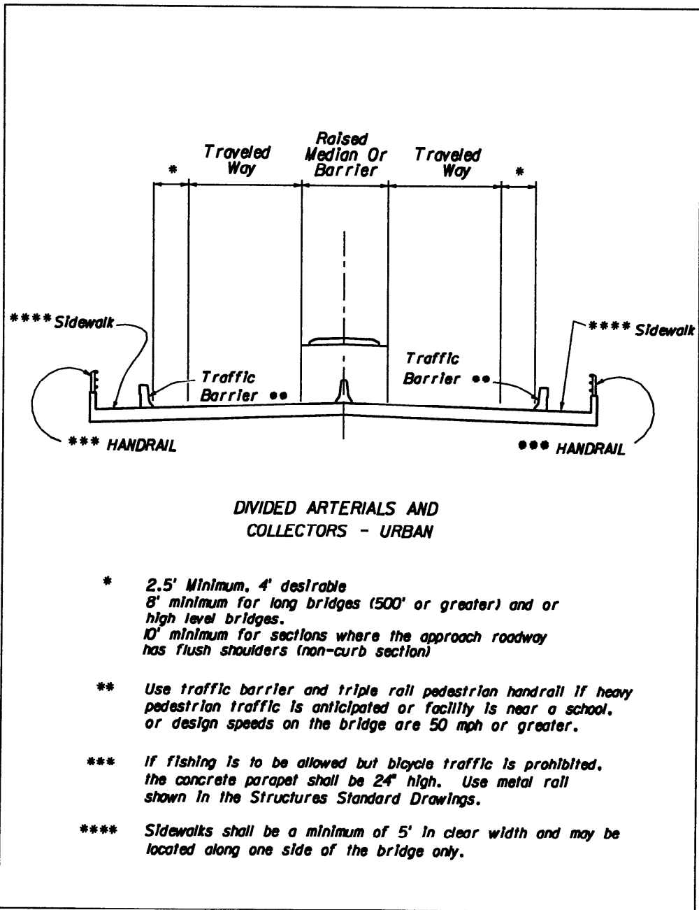
Figure 2.04 Bridge Section
