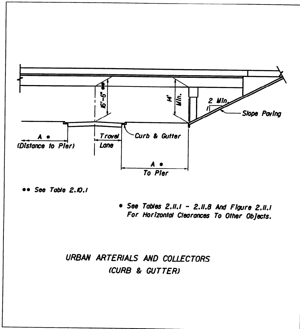
Figure 2.10.4 Clearances
