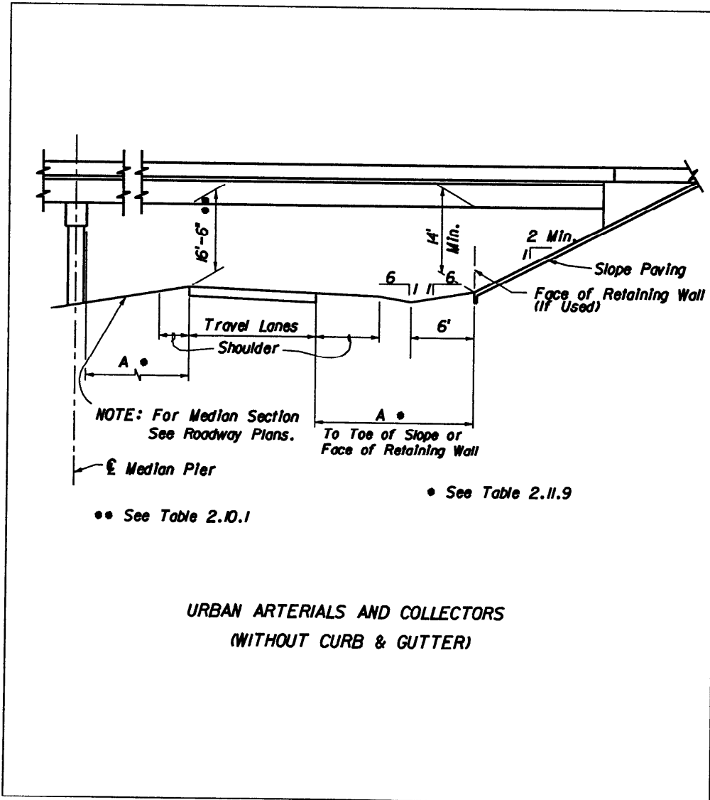
Figure 2.10 3 Clearances
