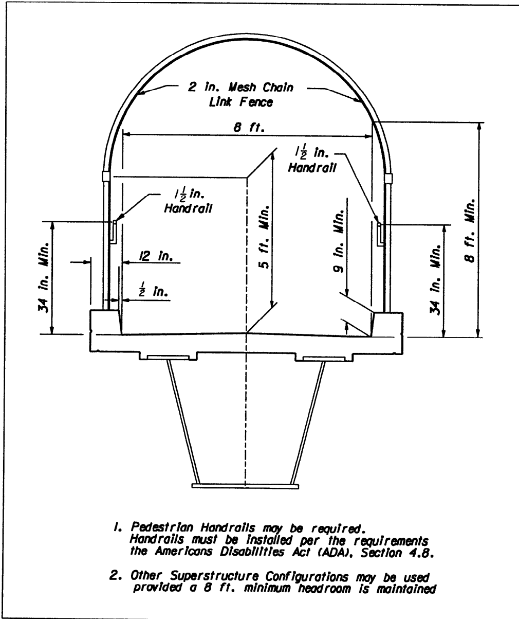
Figure 8-1 Pedestrian Bridge Typical Section
