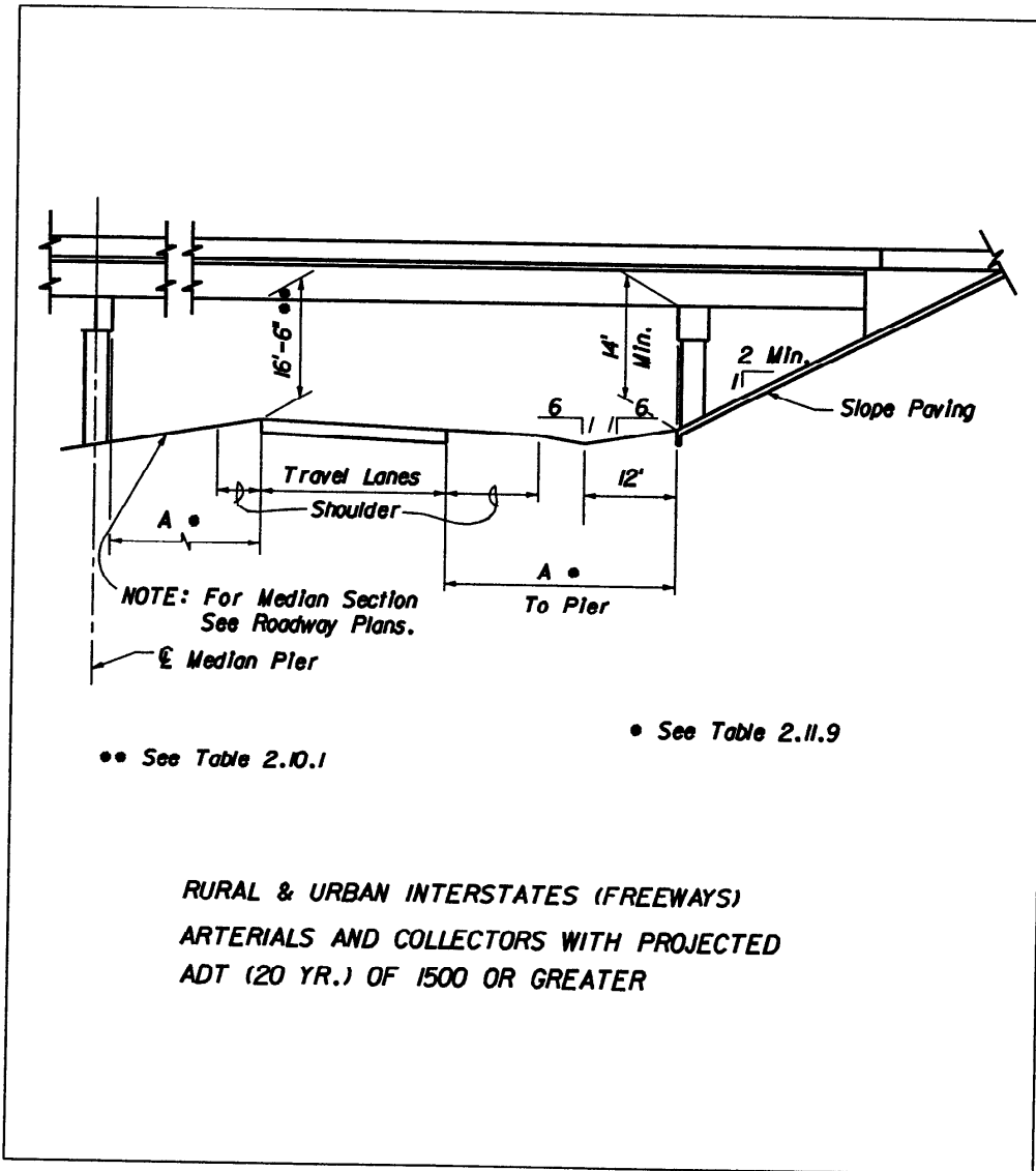
Figure 2.10.1 Clearances
