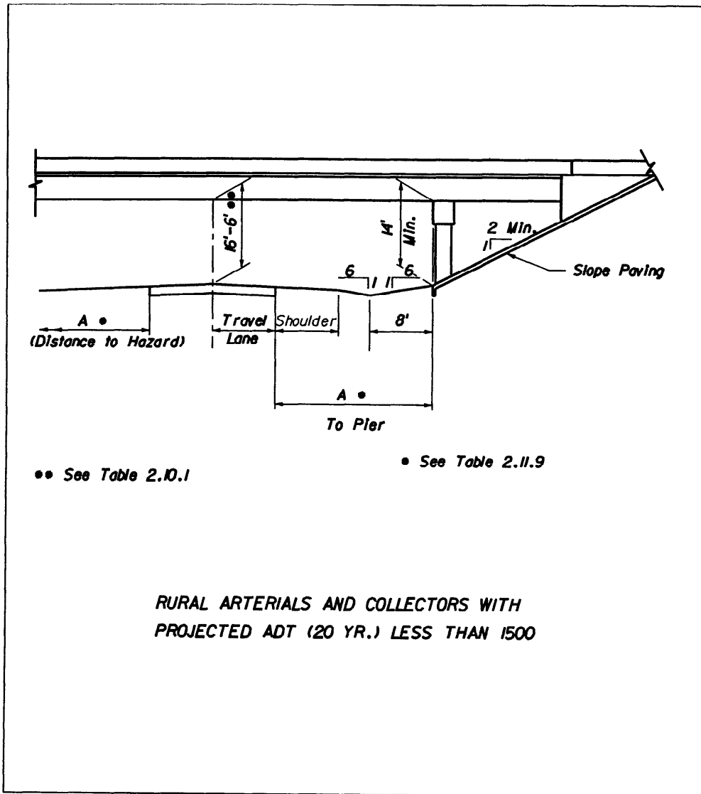
Figure 2 10 2 Clearances
