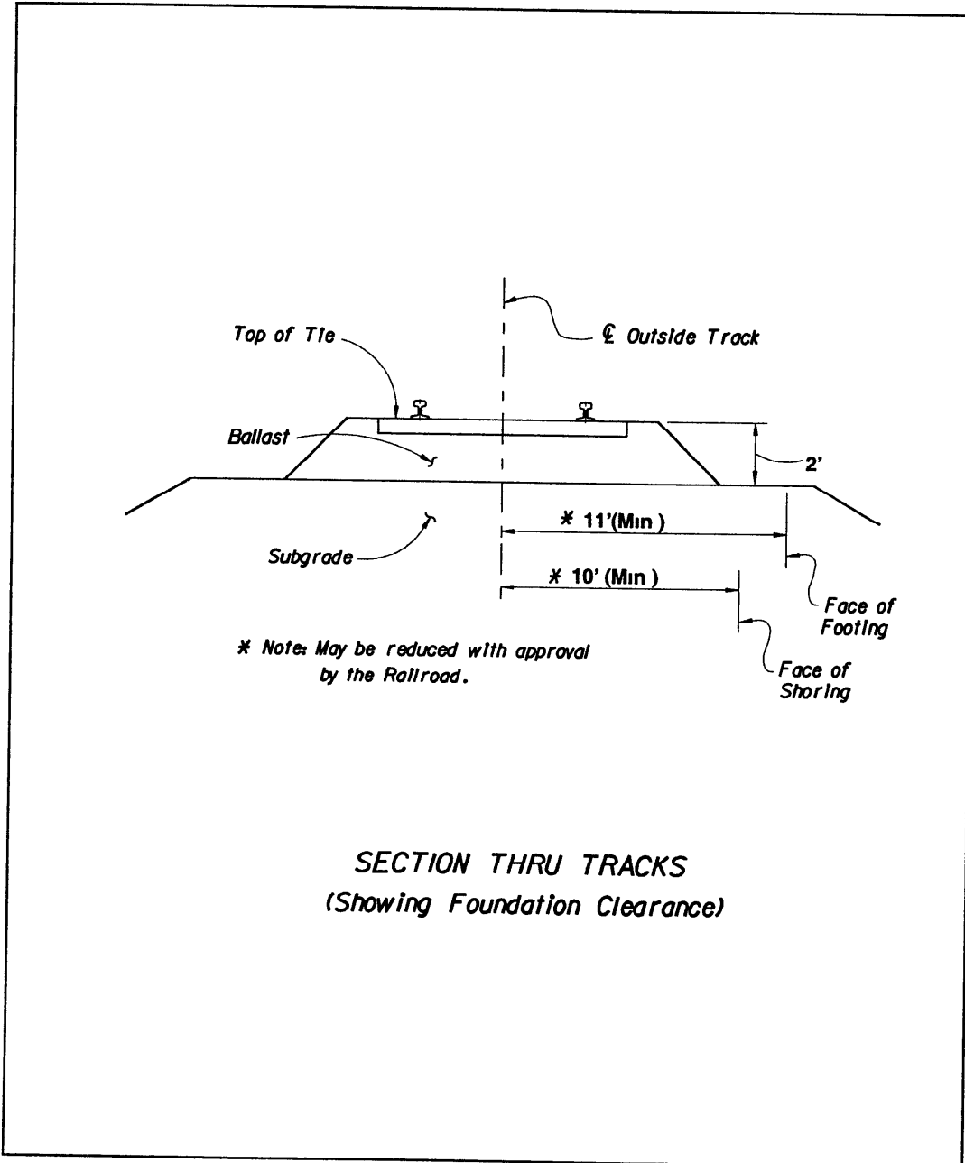
Figure 6.3 Section Thru Tracks
