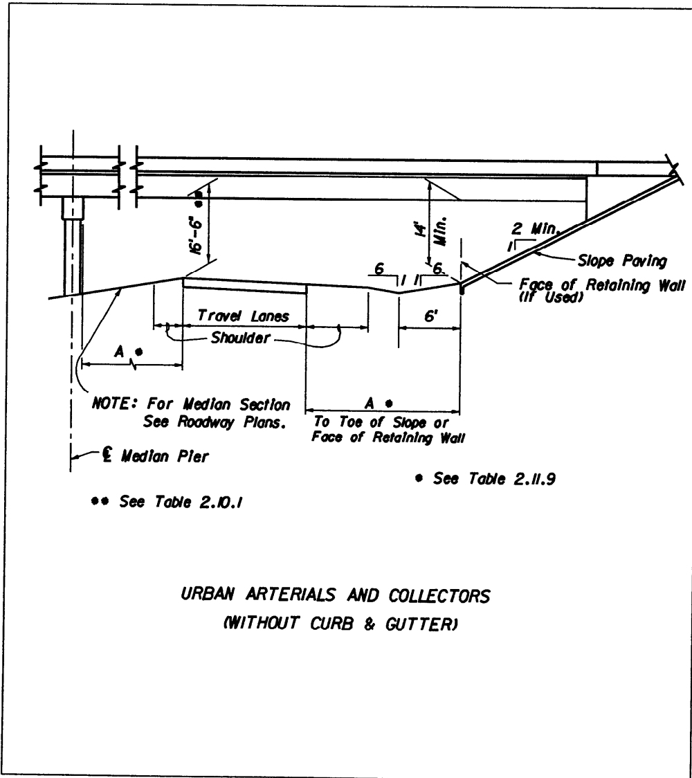
Figure 2 10 3 Clearances
