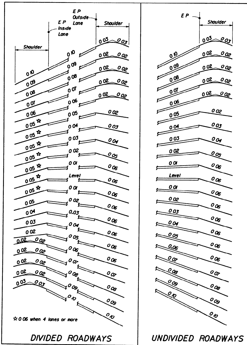
Figure 2.3.1 Shoulder Superelevation
