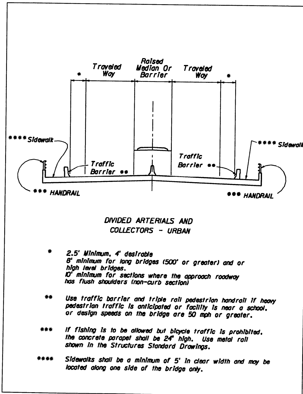
Figure 2.0.4 Bridge Section
