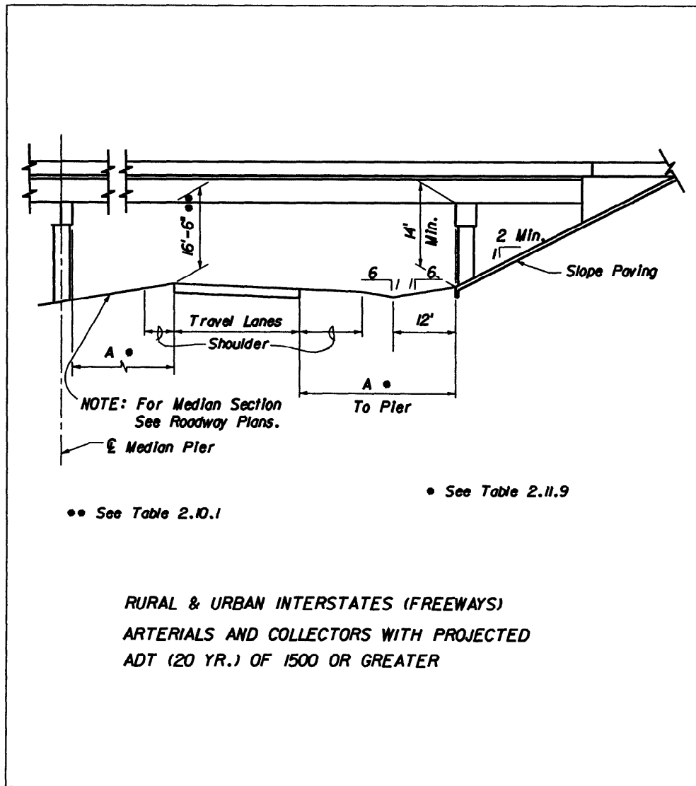
Figure 2.10.1 Clearances
