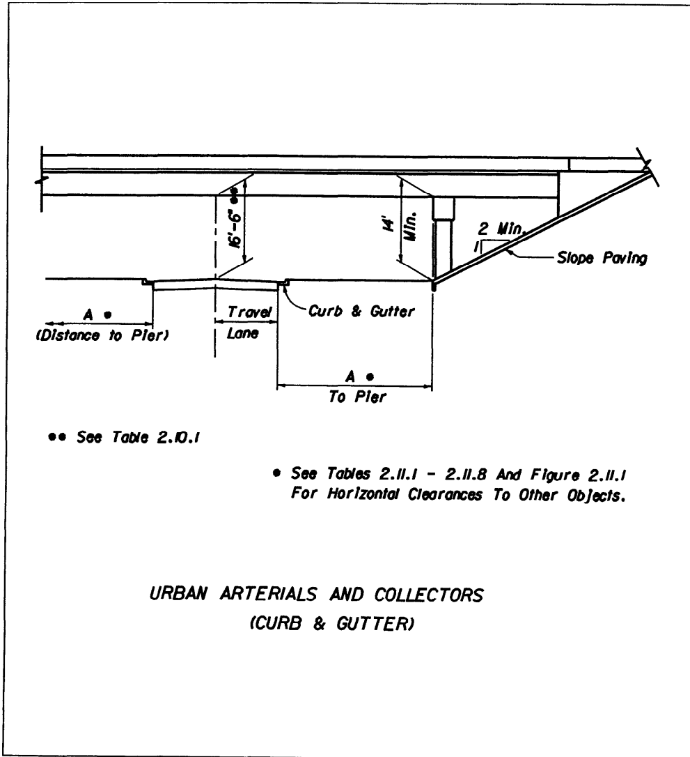
Figure 2.10.4 Clearances
