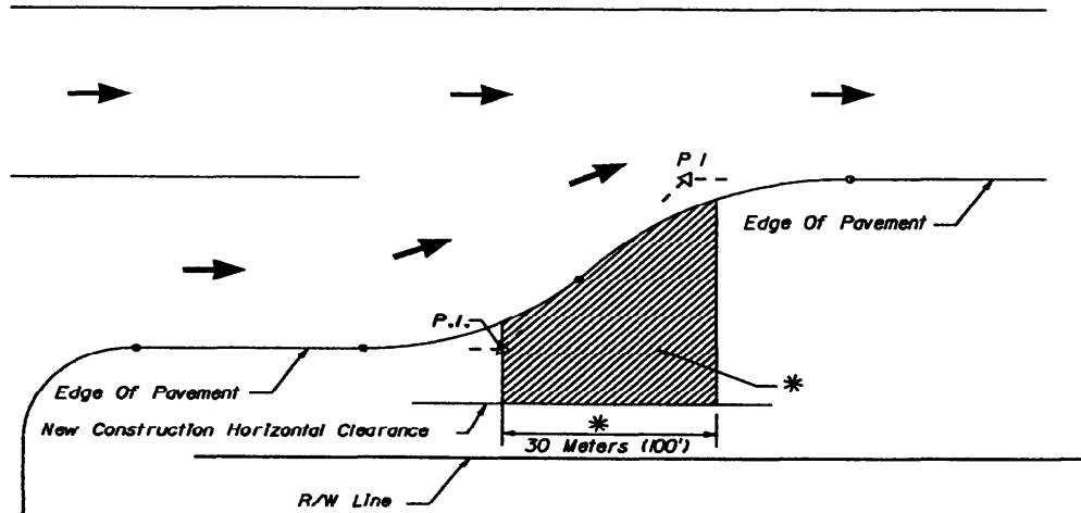
Lane Termination Using A Reverse Curve
