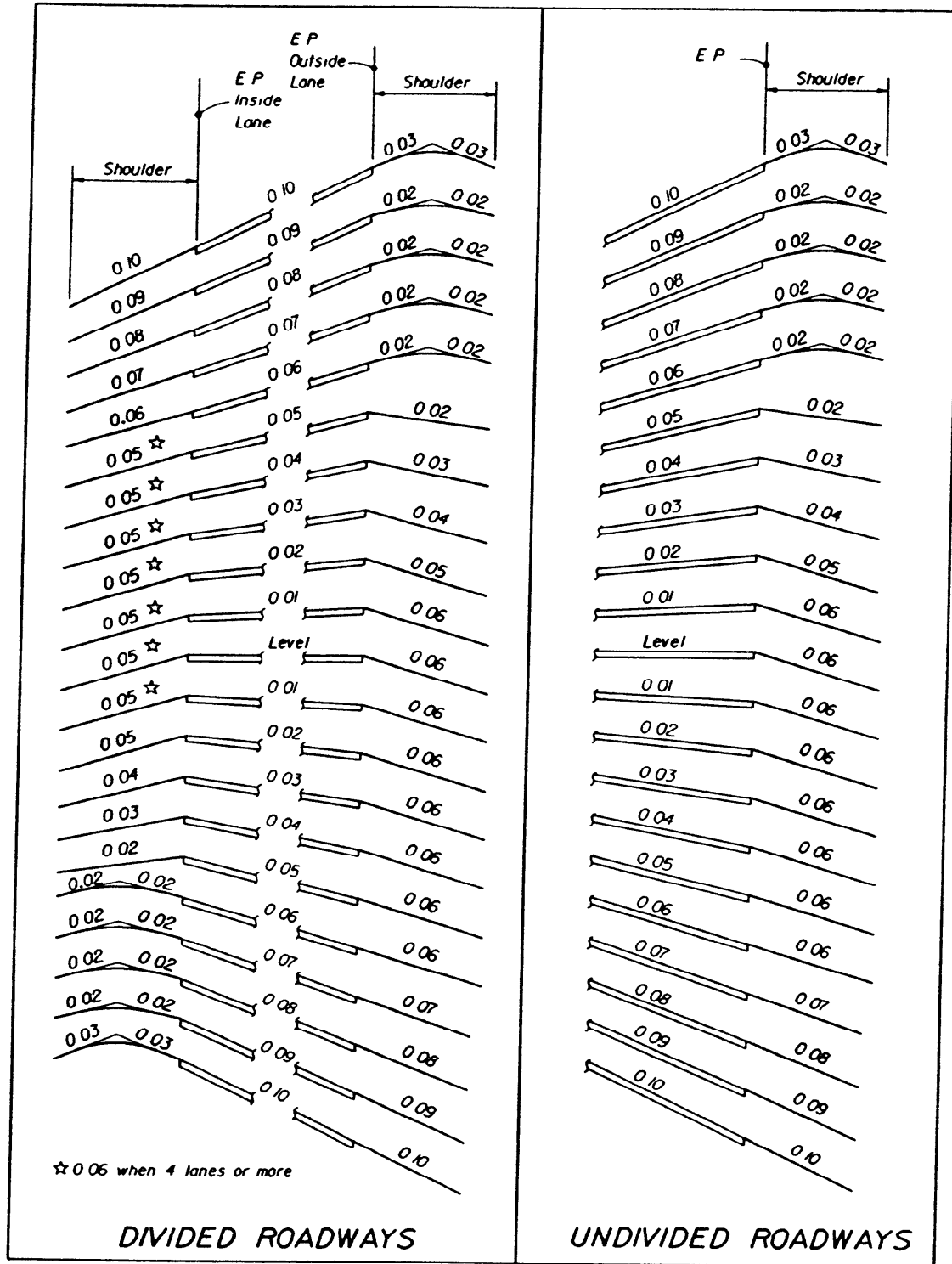
SHOULDER SUPERELEVATION
