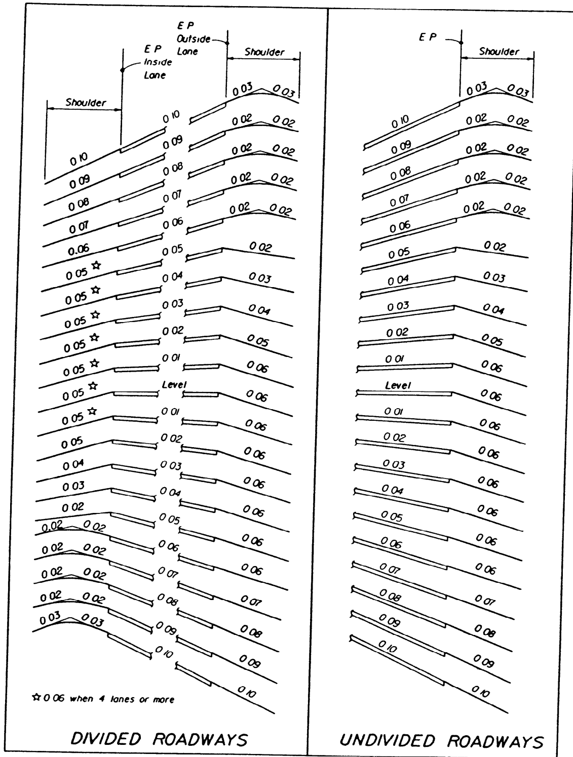
SHOULDER SUPERELEVATION
