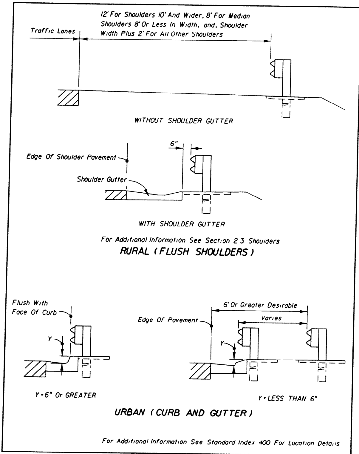
HORIZONTAL CLEARANCE TO GUARDRAIL Figure 2.11.1
