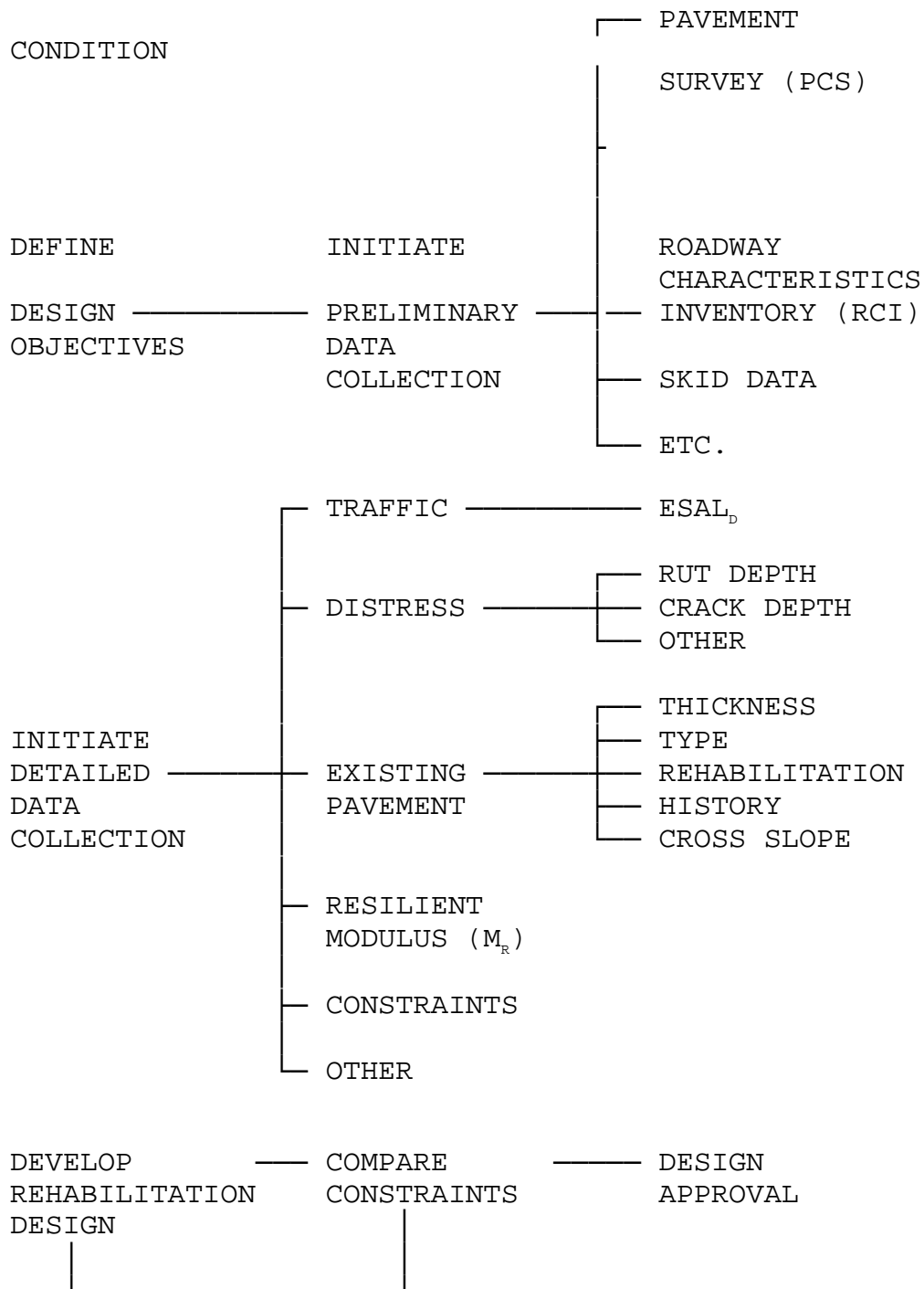
FIGURE 6.1 FLEXIBLE PAVEMENT REHABILITATION PROCESS
