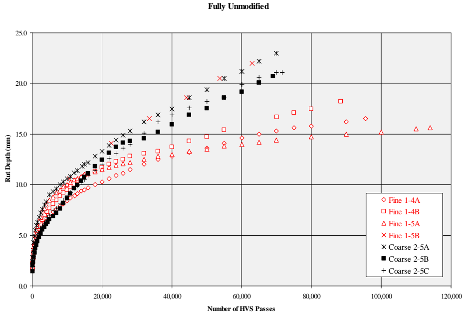
FIGURE 3 Rutting Performance of Fully Unmodified Mixtures.
