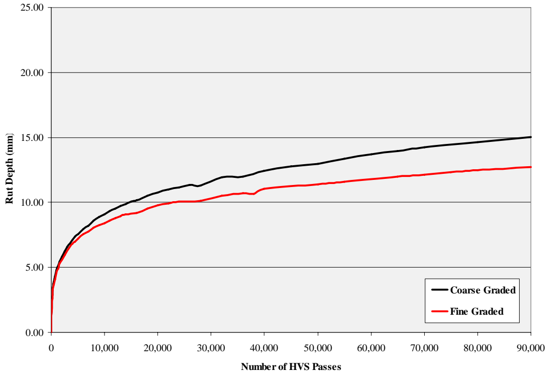
FIGURE 9 Average Rutting Performance of Coarse and Fine Graded Superpave Mixtures.
