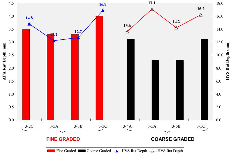
FIGURE 10 APA Test Results (75 mm Specimens)
