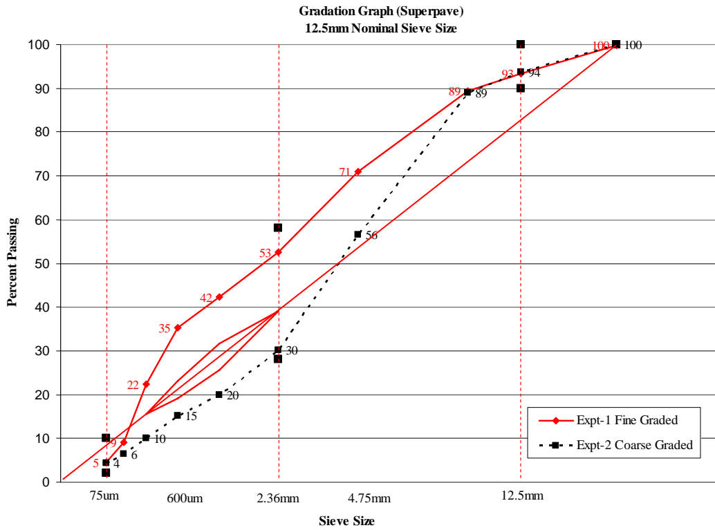
FIGURE 2 Gradation Plot of Coarse and Fine Graded Mixtures from Experiments 1 and 2.
