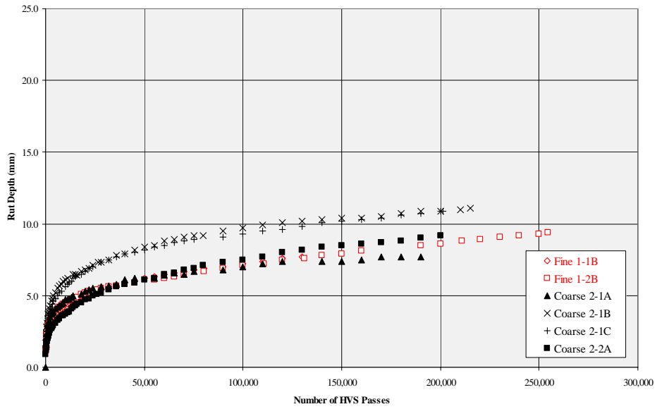
FIGURE 5 Rutting Performance of Fully Modified Mixtures.
