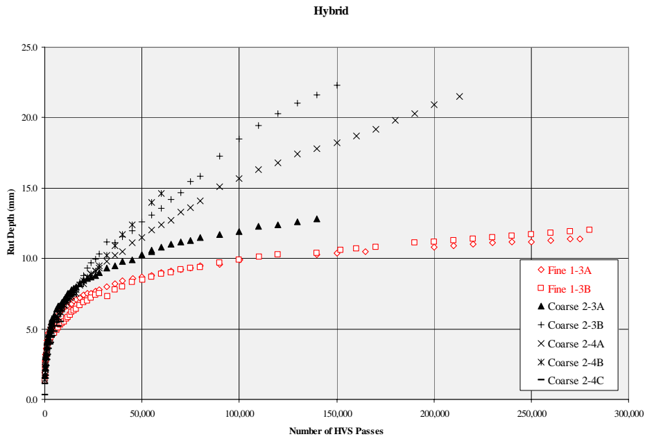
FIGURE 4 Rutting Performance of Hybrid Mixtures.
