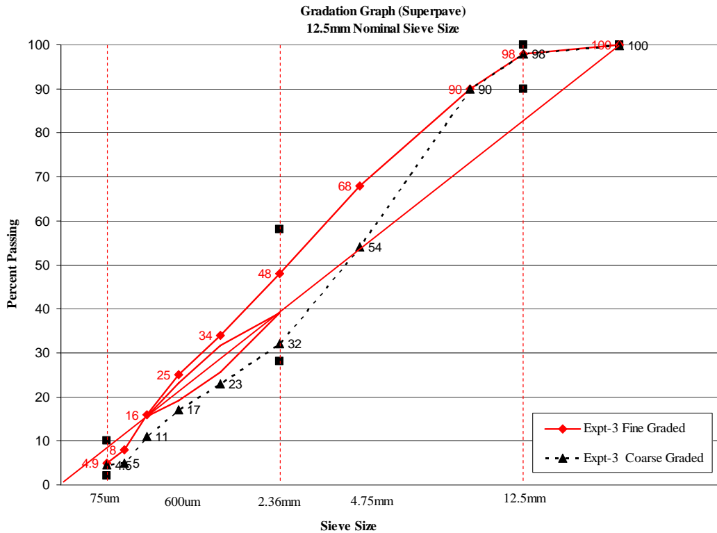
FIGURE 6 Gradation Plot of Coarse and Fine Graded Mixtures from Experiment 3.
