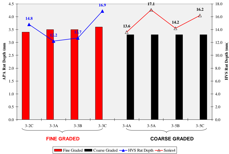
FIGURE 11 APA Test Results (115 mm Specimens)
