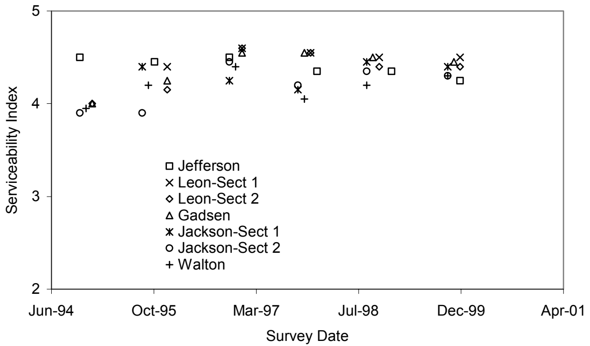
Figure 3 Ride quality vs. time as measured on the westbound direction
