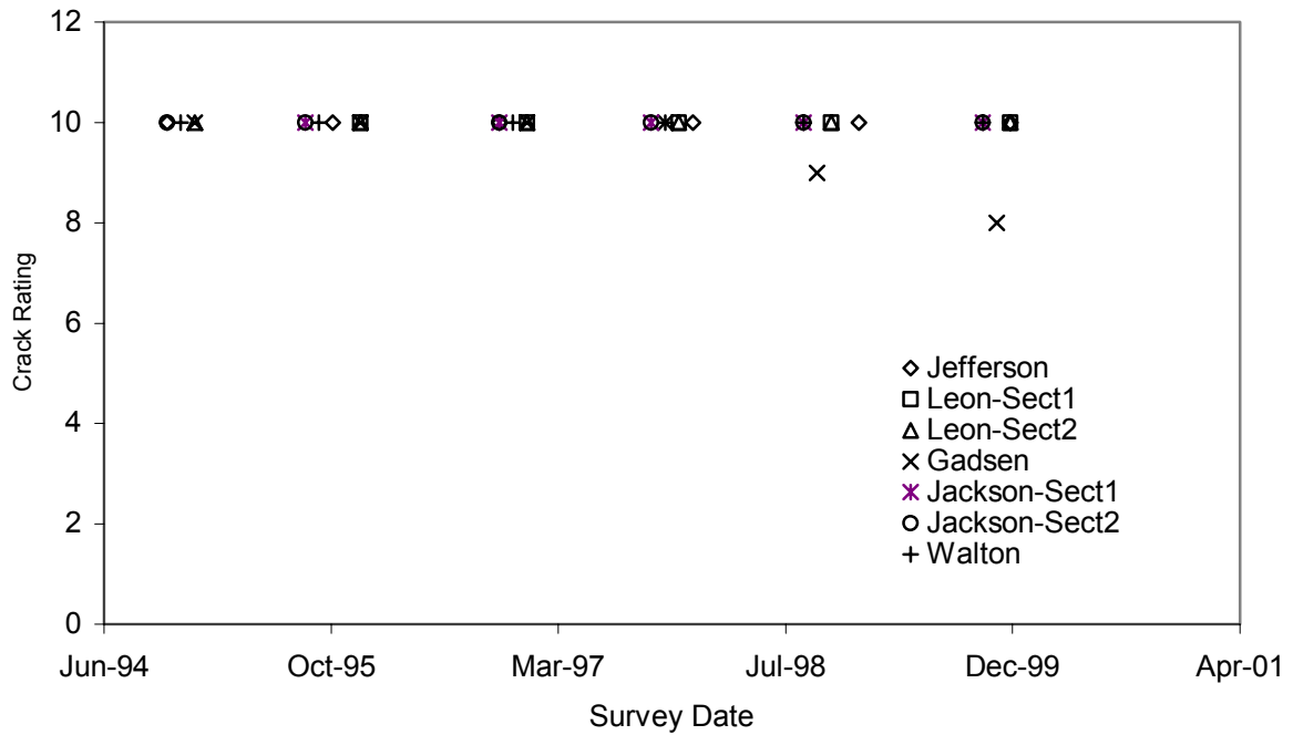
Figure 6 Crack rating vs. time as measured on the eastbound direction
