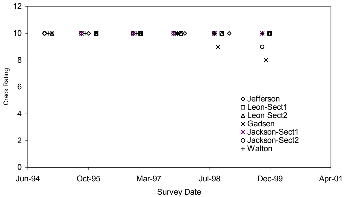
Figure 7 Crack rating vs. time as measured on the westbound direction
