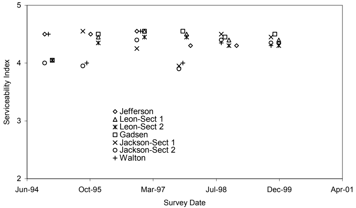
Figure 2 Ride quality vs. time as measured on the eastbound direction
