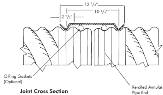
Joint Cross Section
